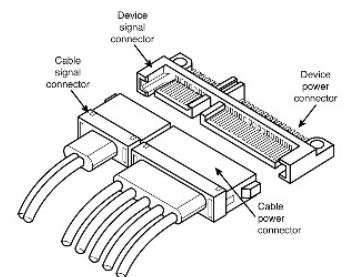
Figure 1 Attaching SATA cabling
