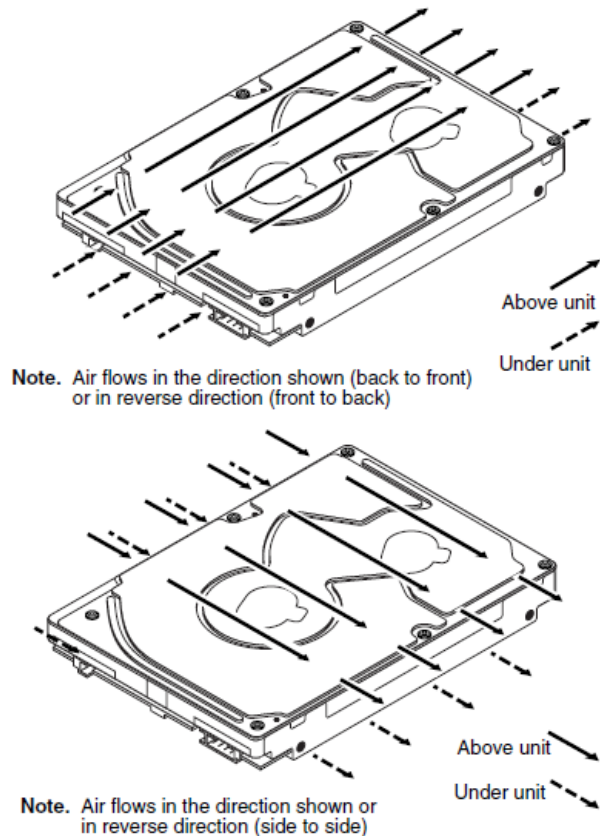
Figure 18. Air flow
