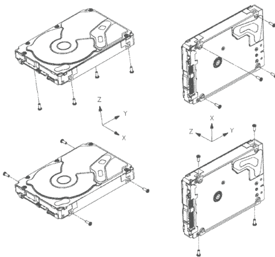
Figure 14. Recommended mounting
