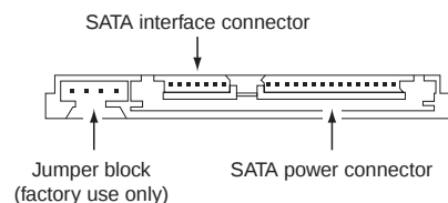
Figure 1. SATA interface and power connectors
