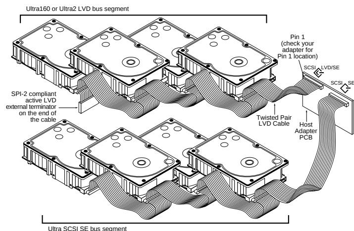
Figure 3. Cable connections and external termination
