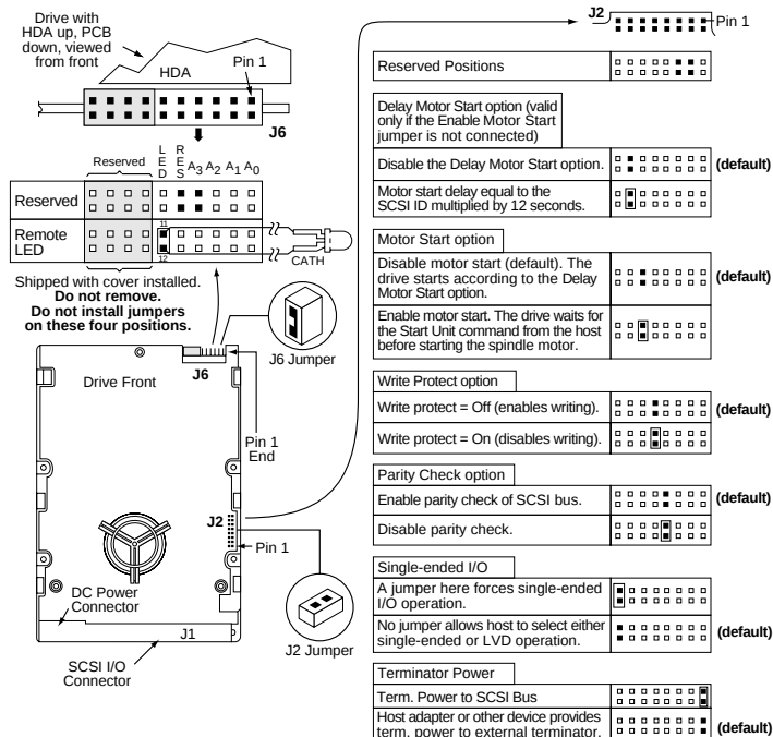
Figure 2. Option select jumpers
