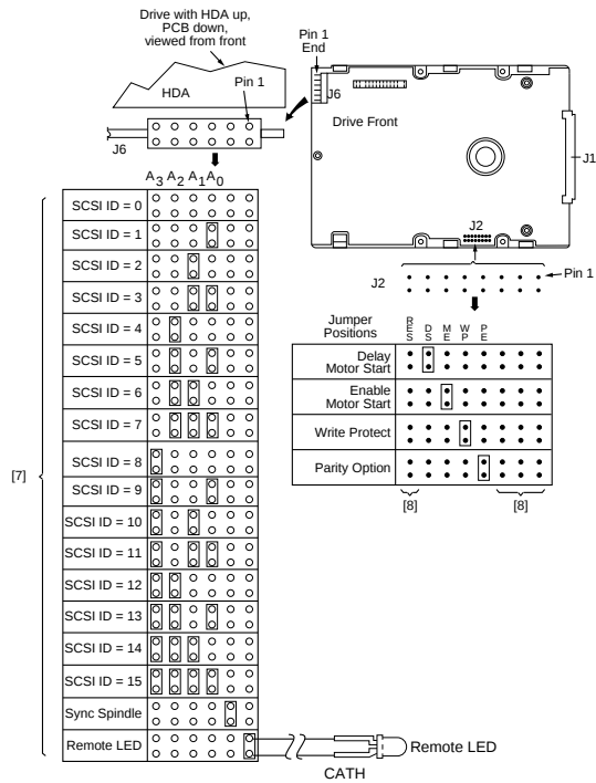
Figure 3c. Drive configurator for Hawk 1LP family WC model
