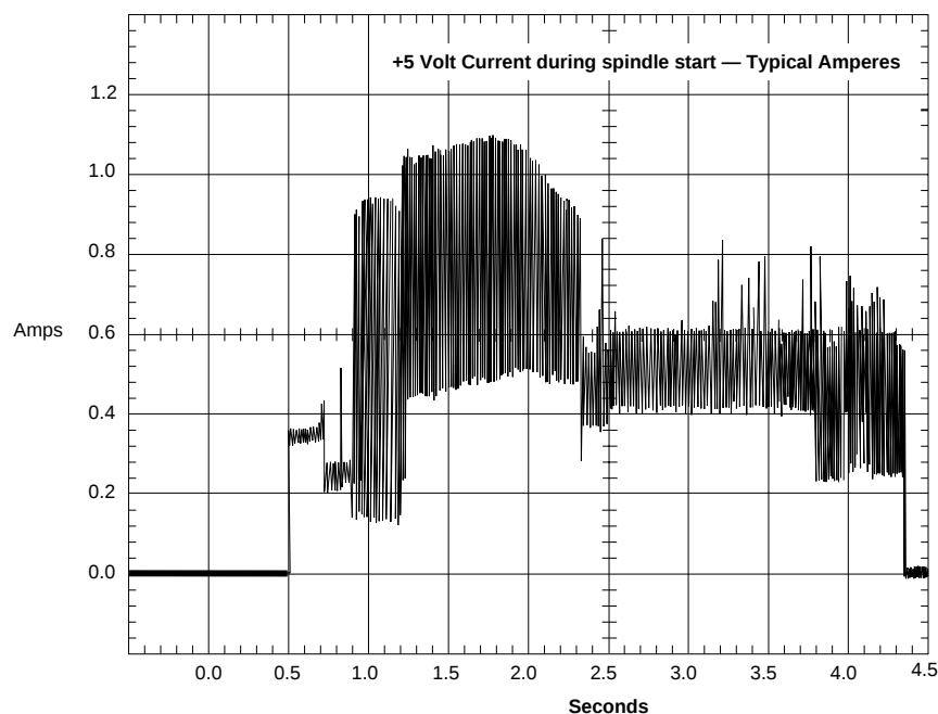
Figure 2. Typical 5V startup and operation current profile
