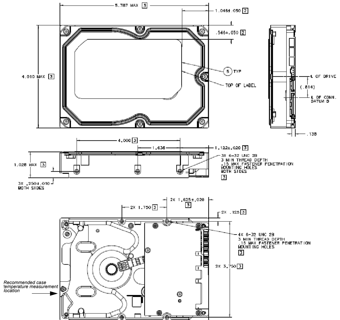
Figure 4. Mounting dimensions (2TB and 1TB)
