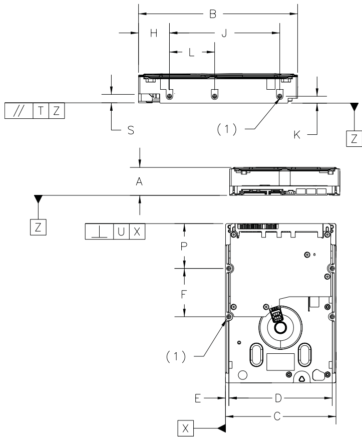
Figure 9. Physical dimensions
