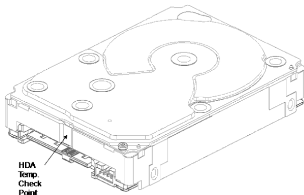
Figure 7. Location of the HDA temperature check point
