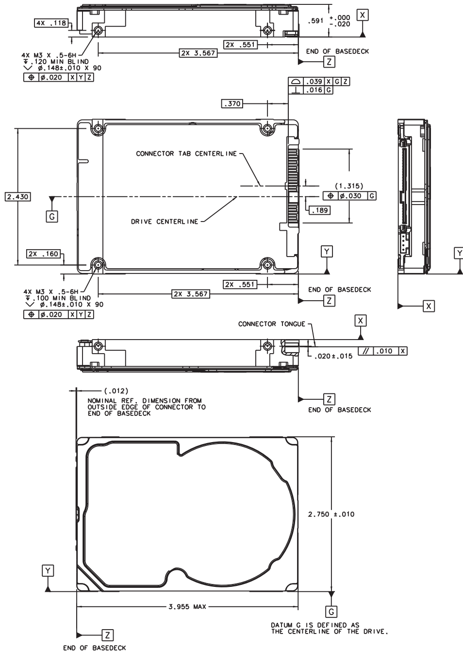
Figure 9. Mounting configuration dimensions
