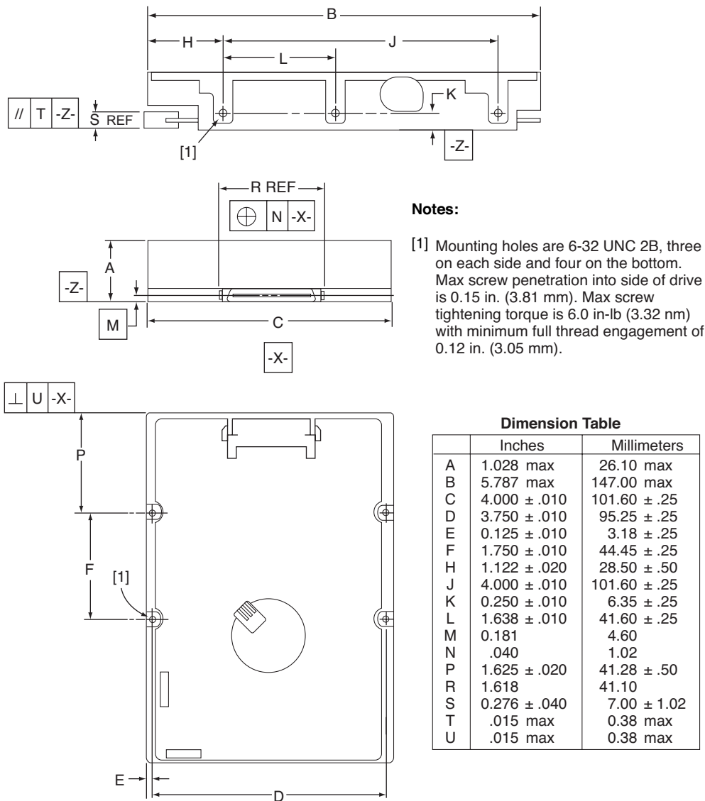
Figure 12. Mounting configuration dimensions
