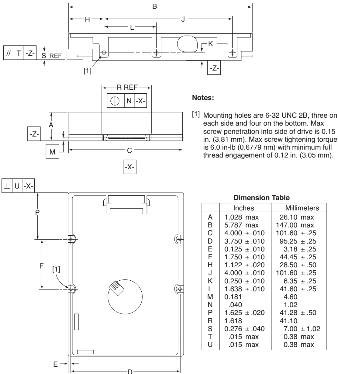
Figure 9. Mounting configuration dimensions
