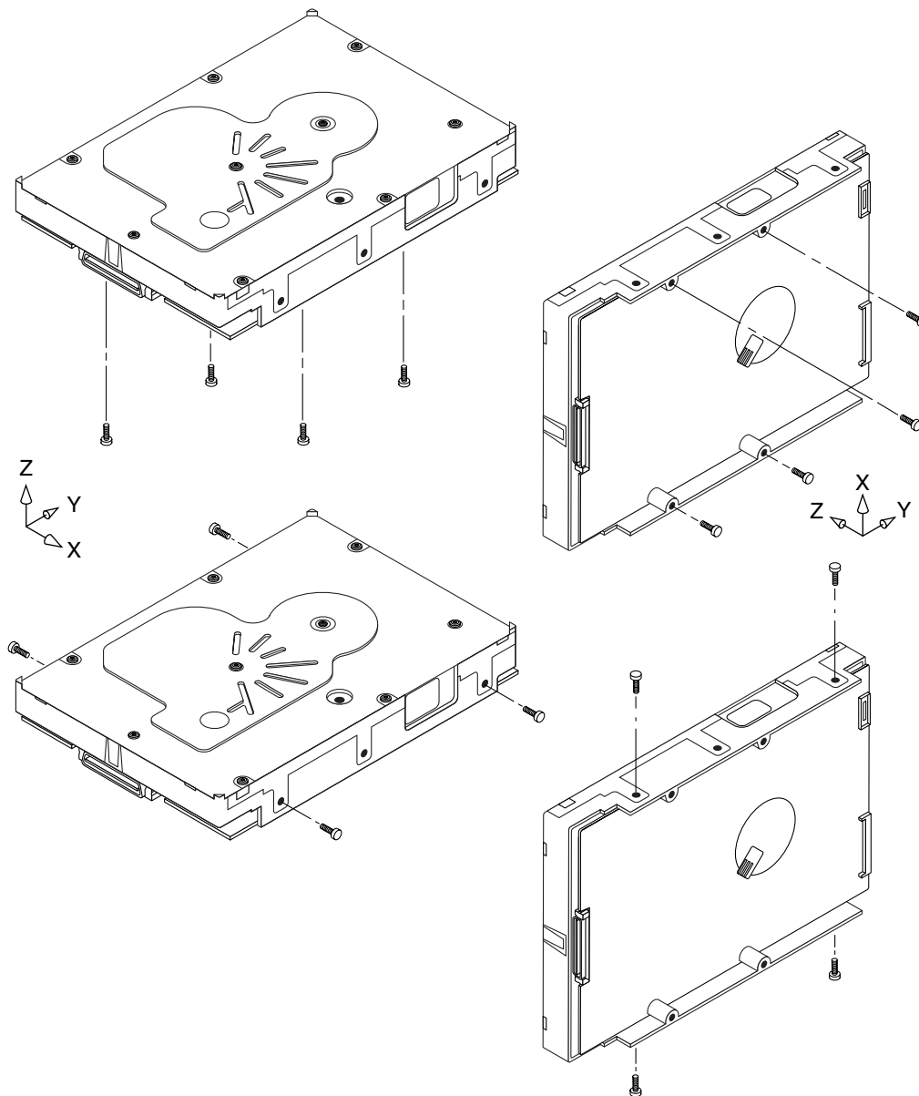
Figure 8. Recommended mounting
