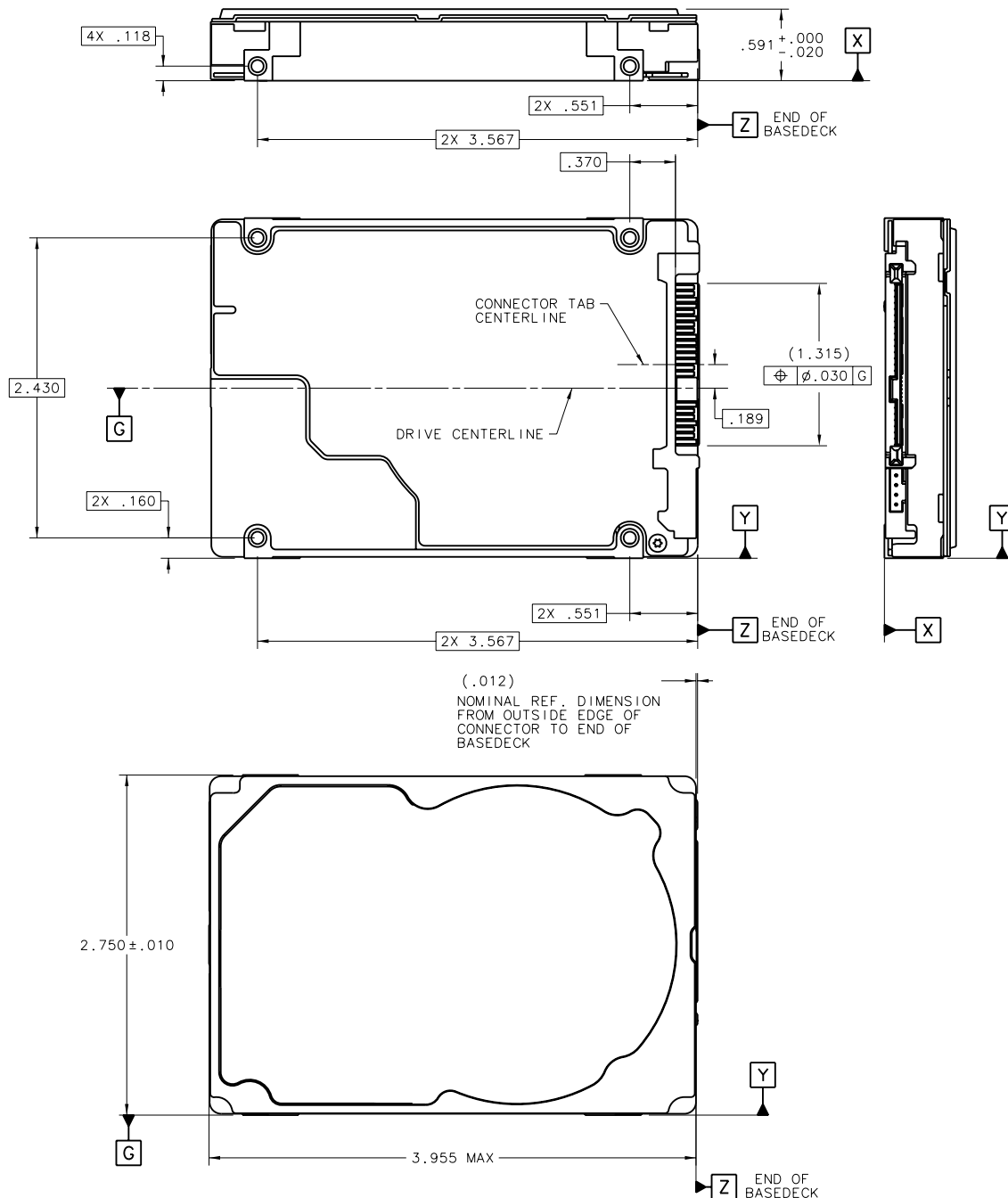
Figure 9. Dimensions
