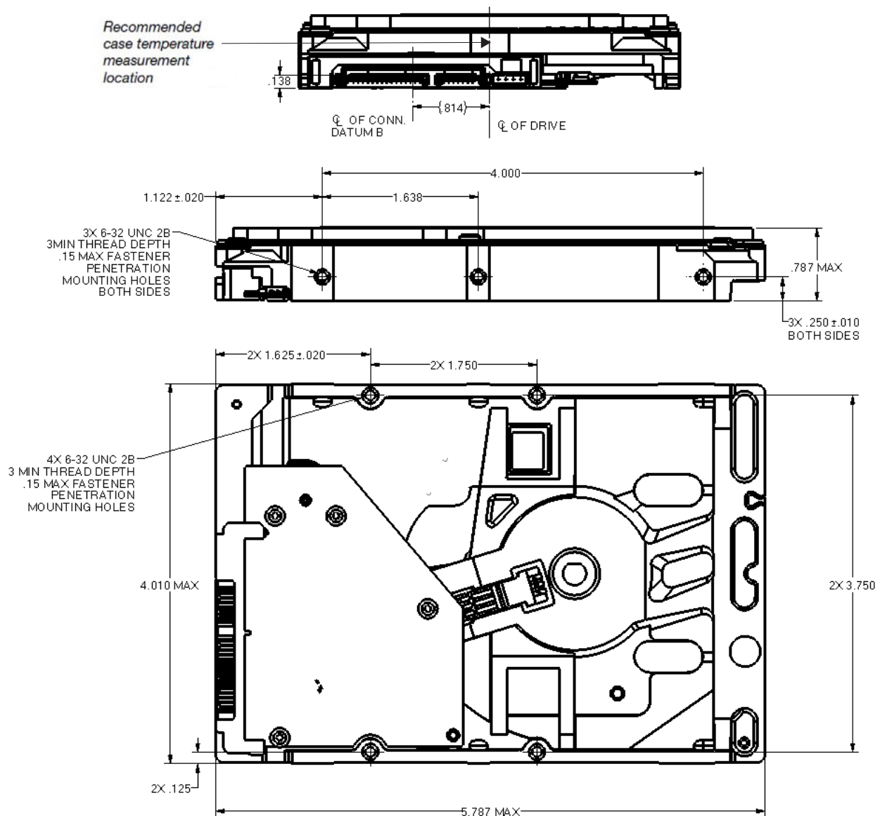
Figure 4 Mounting dimensions (1TB model)
