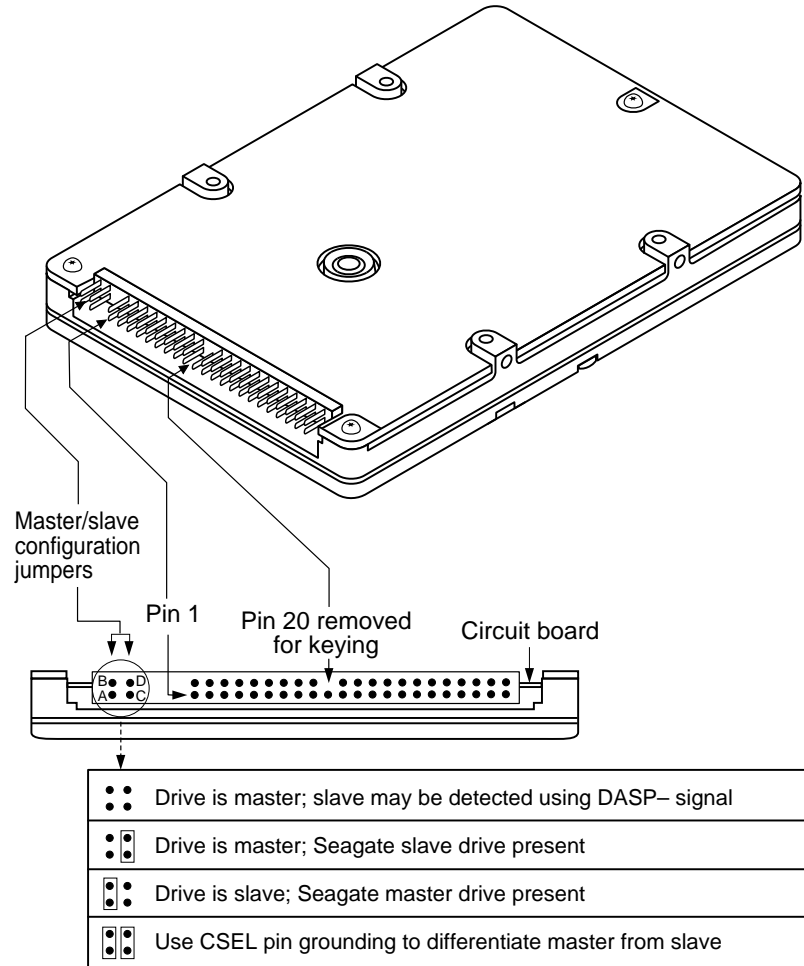
Figure 3. Connector setup for the ST9190 family drives
