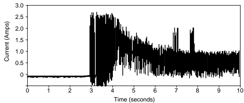
Figure 1. Typical startup and operation current profile
