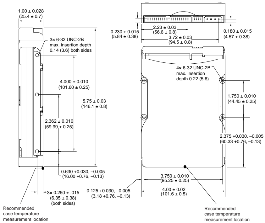
Figure 4. Mounting dimensions—top, side and end view
