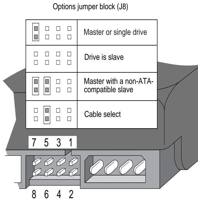
Figure 2. Master/slave jumper settings
