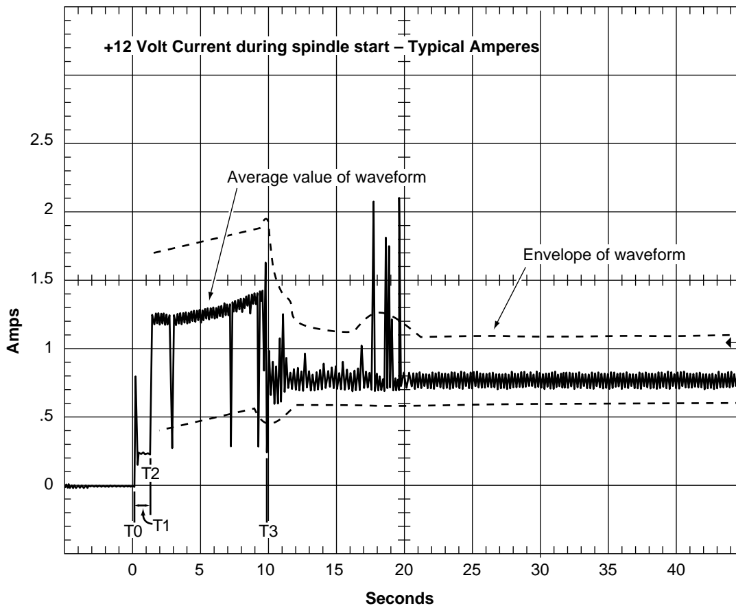
Figure 3. Typical Cheetah 9LP FC drive +12V current profile
