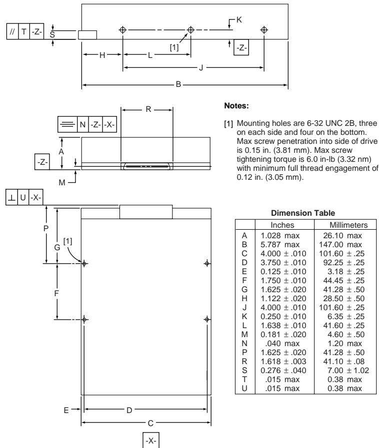
Figure 4. Mounting configuration dimensions
