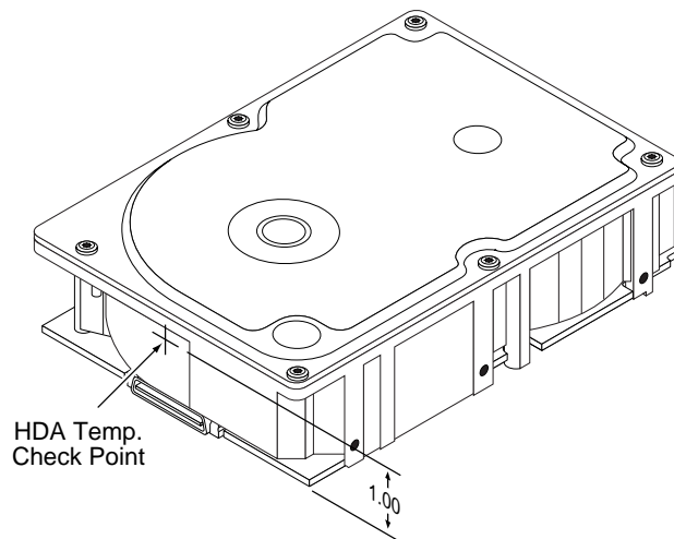
Figure 9. HDA case temperature measurement location
