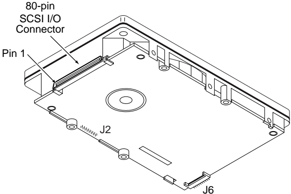
Figure 13. ST39102LC and ST34502LC drive physical interface (80-pin J1 SCSI I/O connector)
