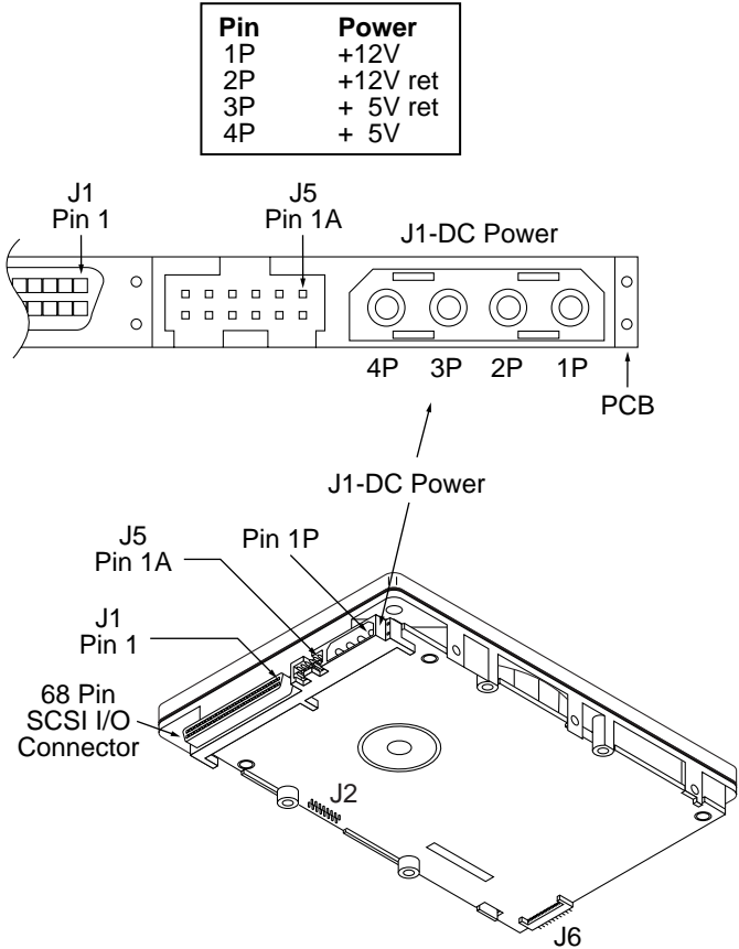
Figure 12. ST39102LW and ST34502LW drive physical interface (68-pin J1 SCSI I/O connector)
