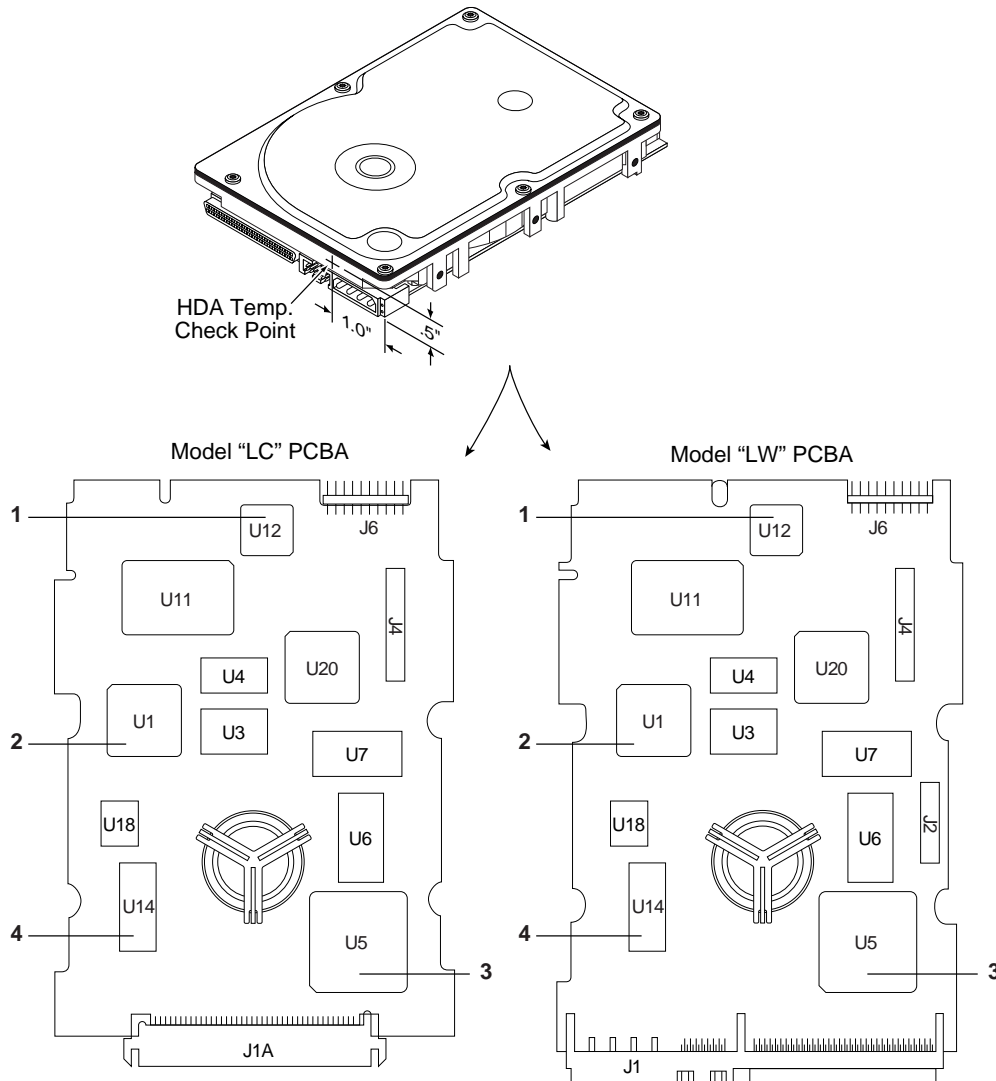
Figure 4. Locations of PCBA components listed in Table 3
