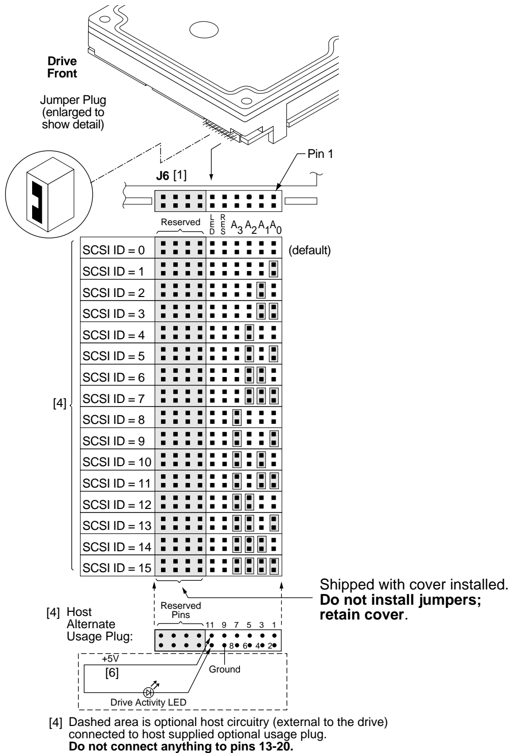
Figure 8. J6 jumper header
