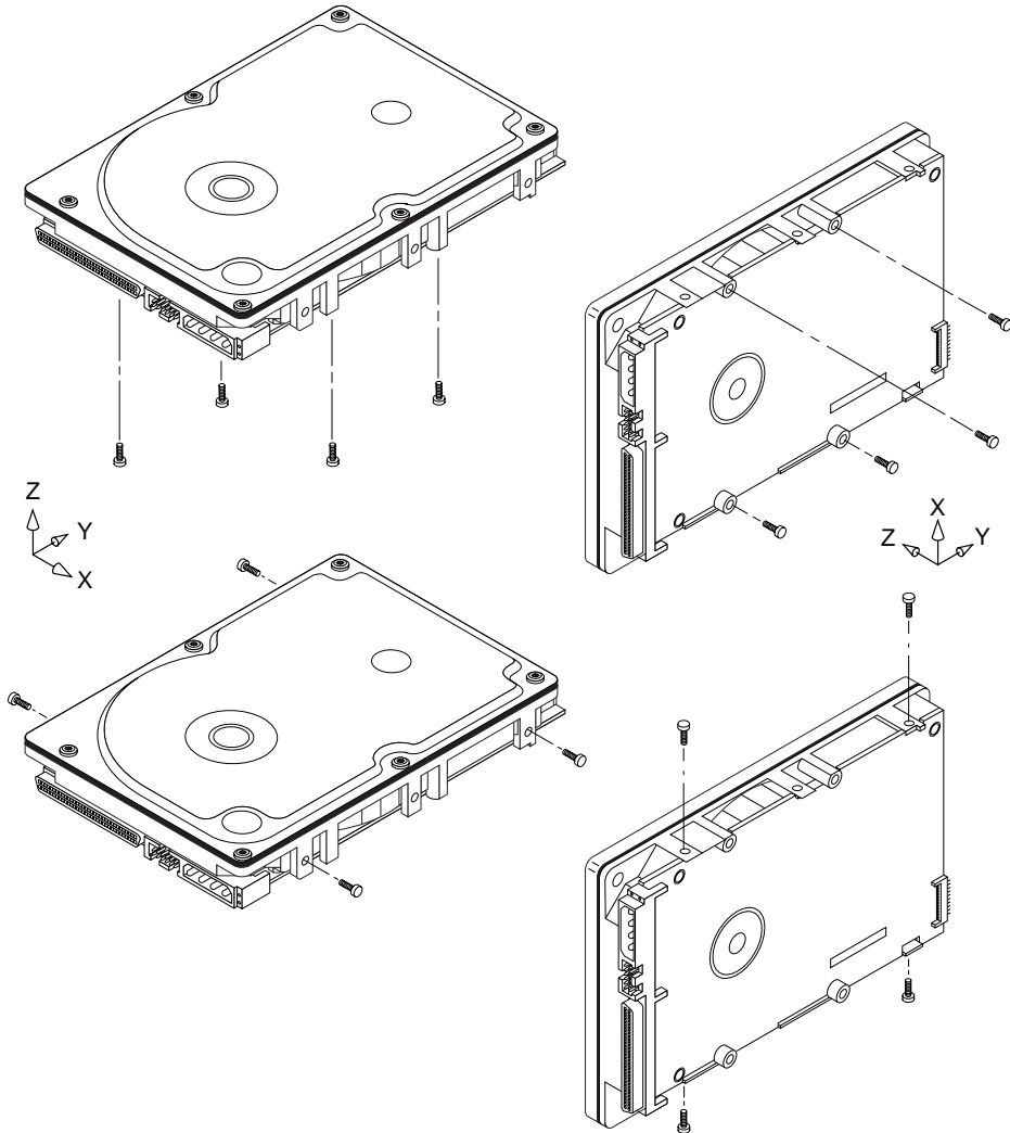
Figure 5. Recommended mounting
