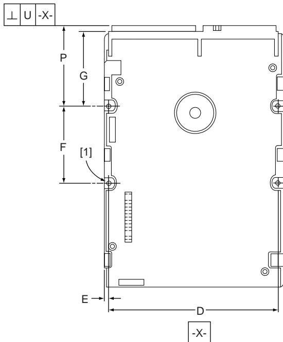
Figure 6. ST39102LW and ST34502LW mounting configuration dimensions
