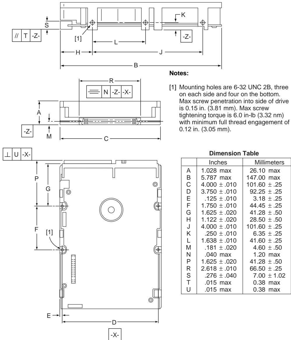
Figure 7. ST39102LC and ST34502LC mounting configuration dimensions
