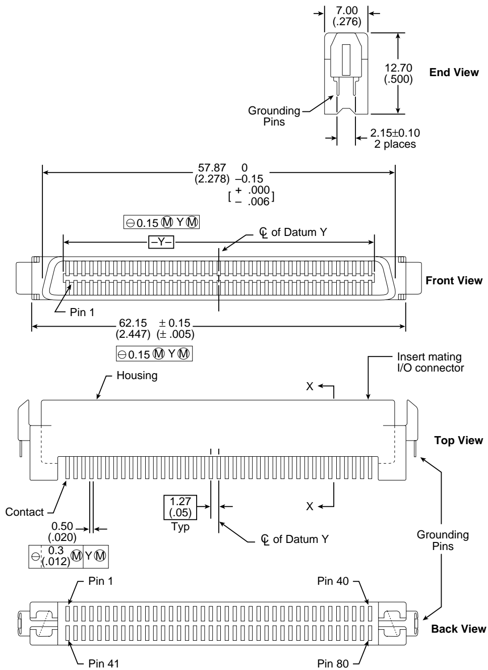
Figure 16. Nonshielded 80 pin SCSI "SCA-2" connector, used on LC drives
