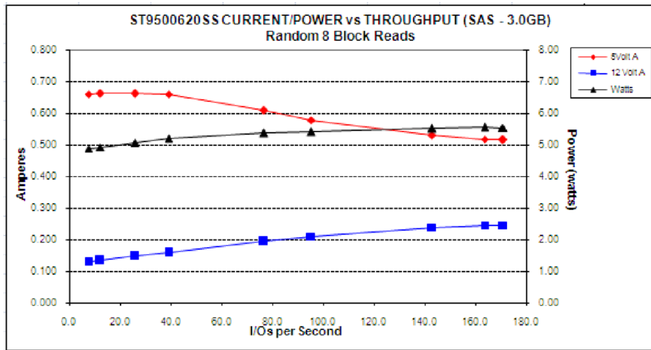
Figure 5. 500GB Models (3Gb) DC current and power vs. input/output operations per second
