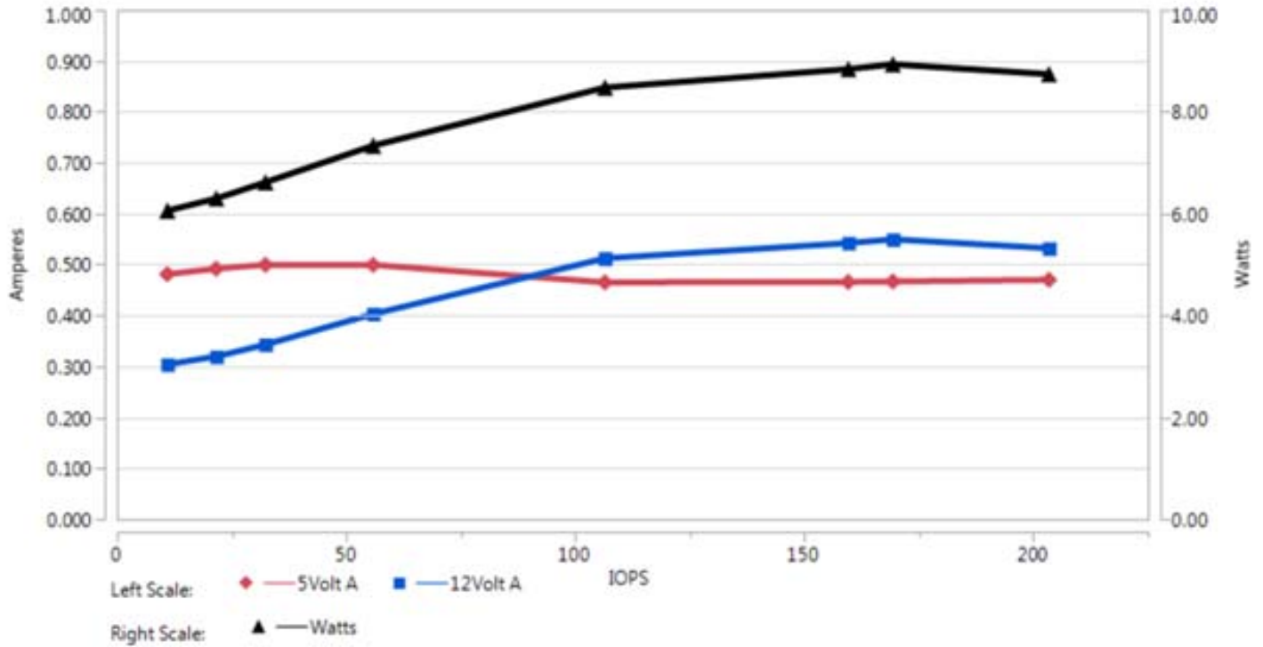
Figure 2. 10TB models (12Gb) DC current and power vs. input/output operations per second
