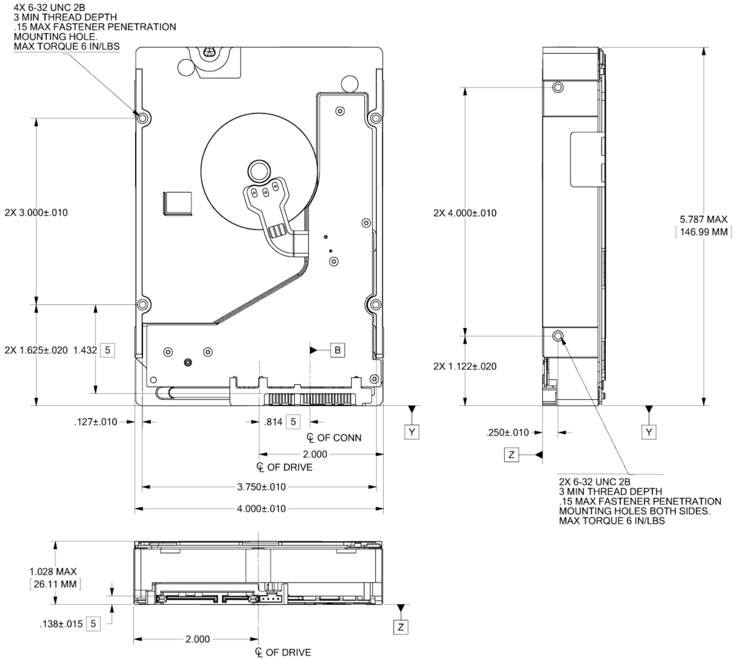
Figure 5. Mounting configuration dimensions (10TB models)
