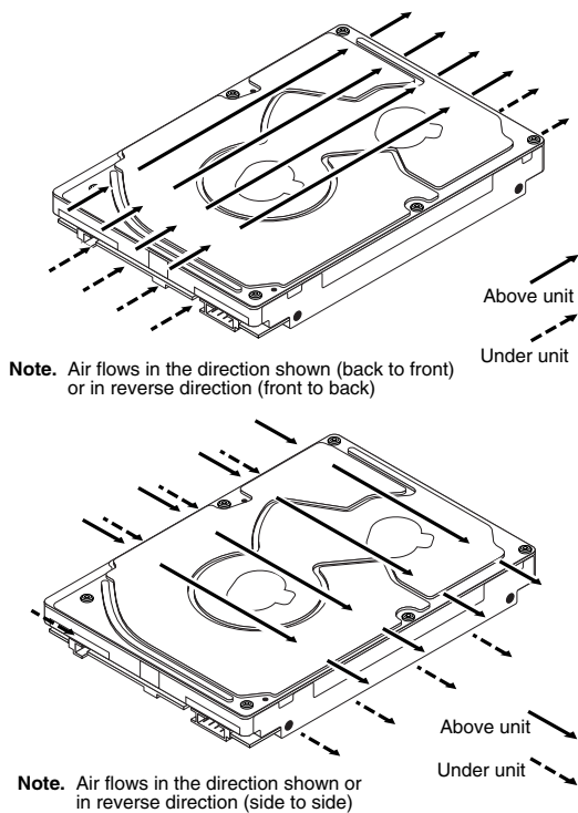
Figure 18. Air flow
