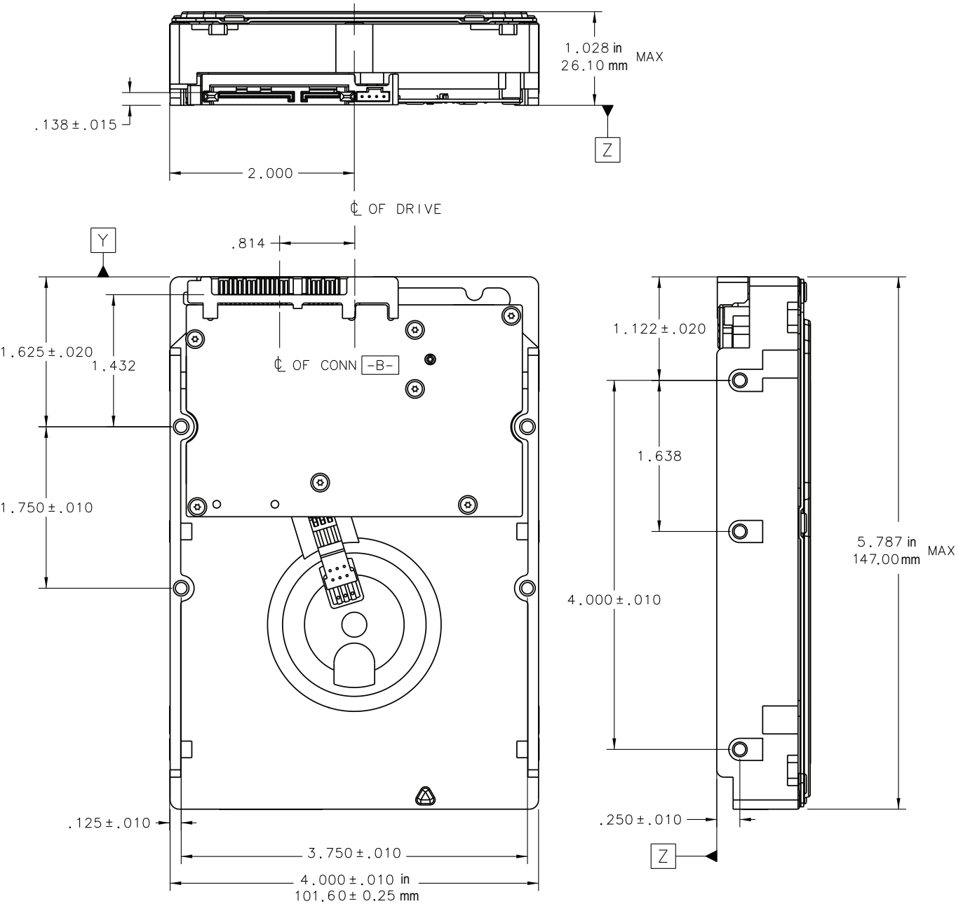
Figure 15. Mounting configuration dimensions
