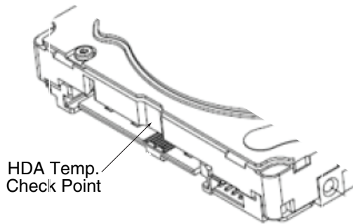
Figure 13. Location of the HDA temperature check point
