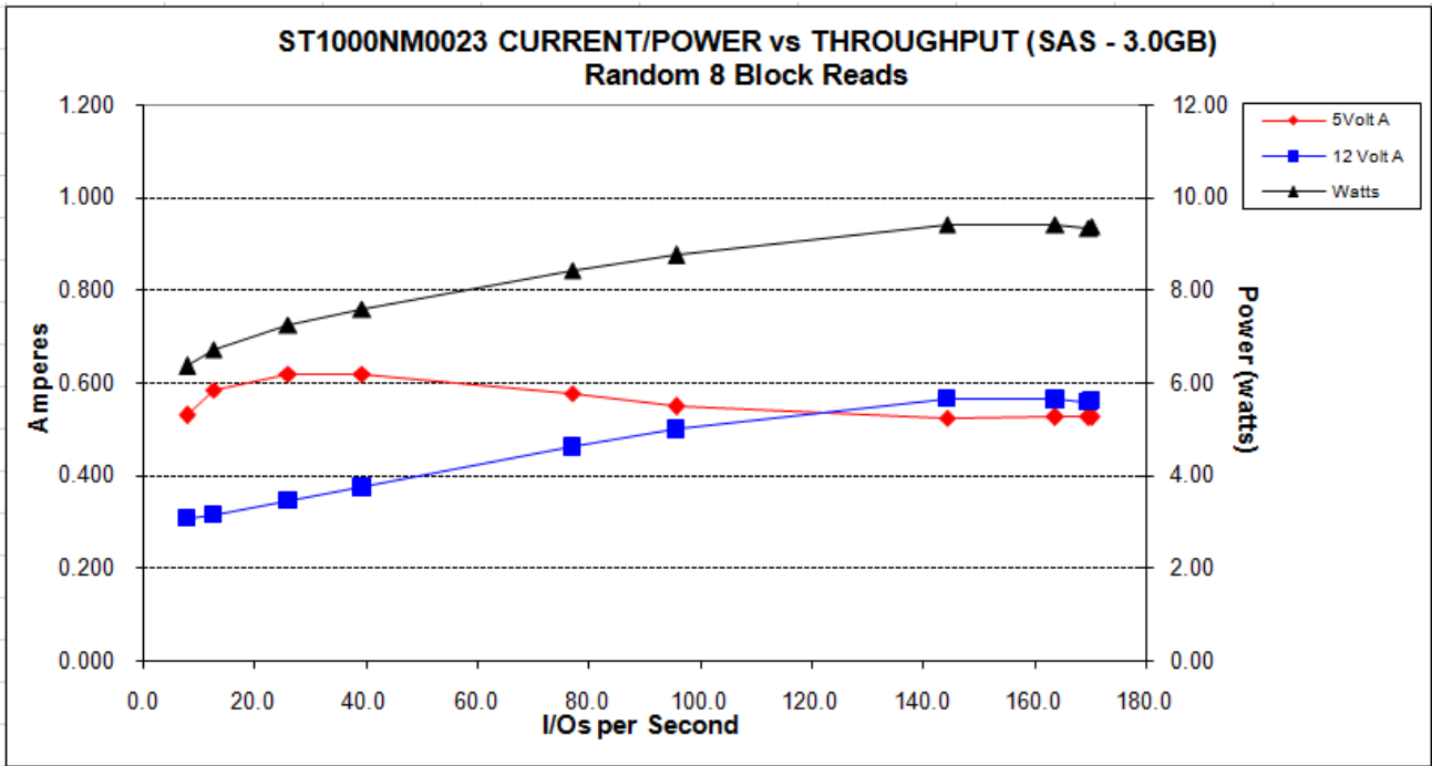
Figure 11. 1TB models (3Gb) DC current and power vs. input/output operations per second
