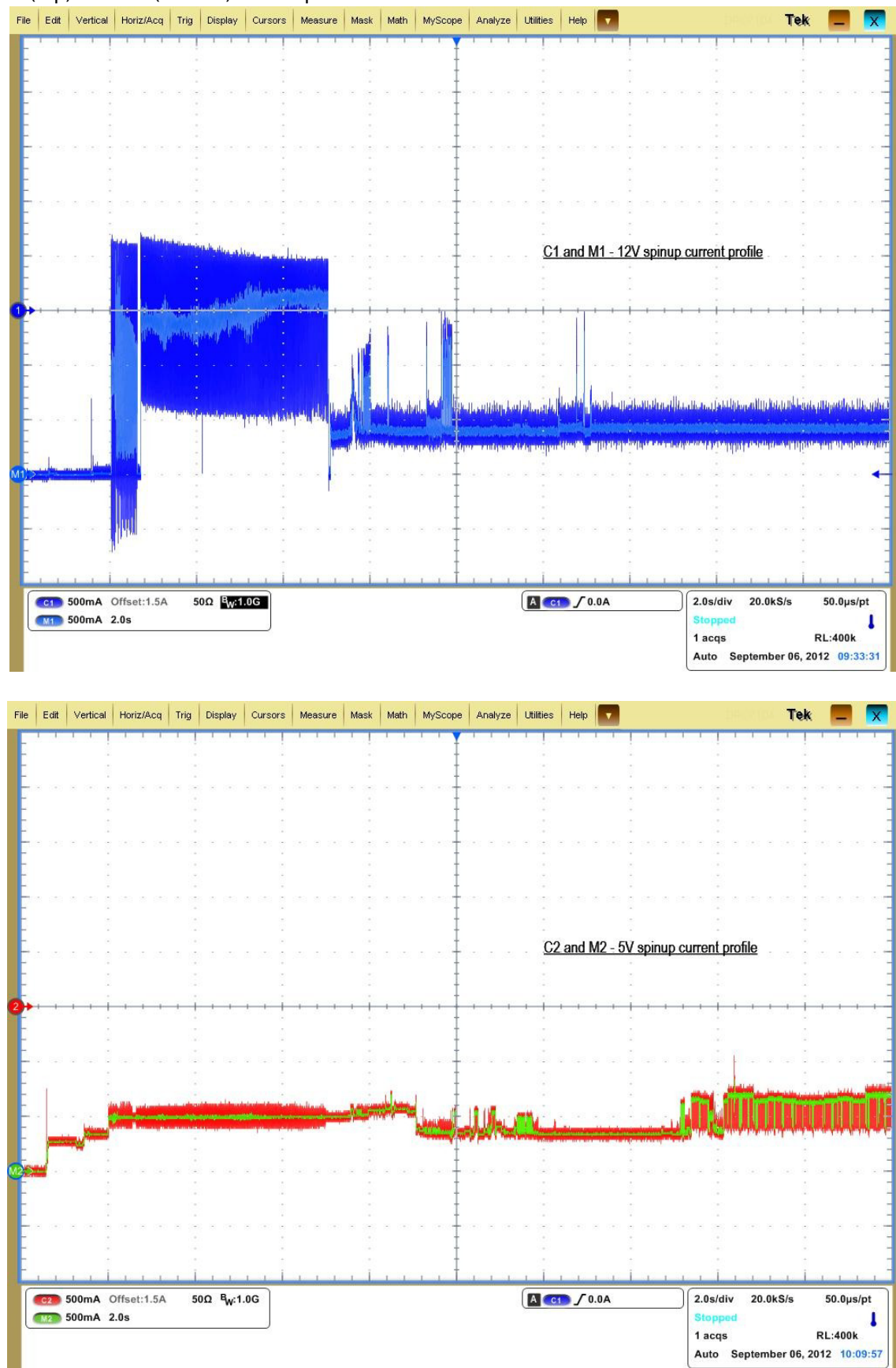
Figure 3. 2TB model current profiles
