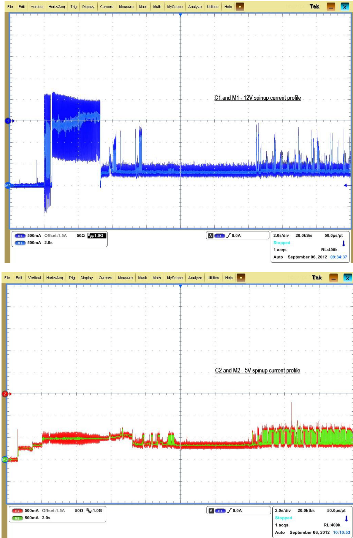
Figure 4. 1TB model current profiles
