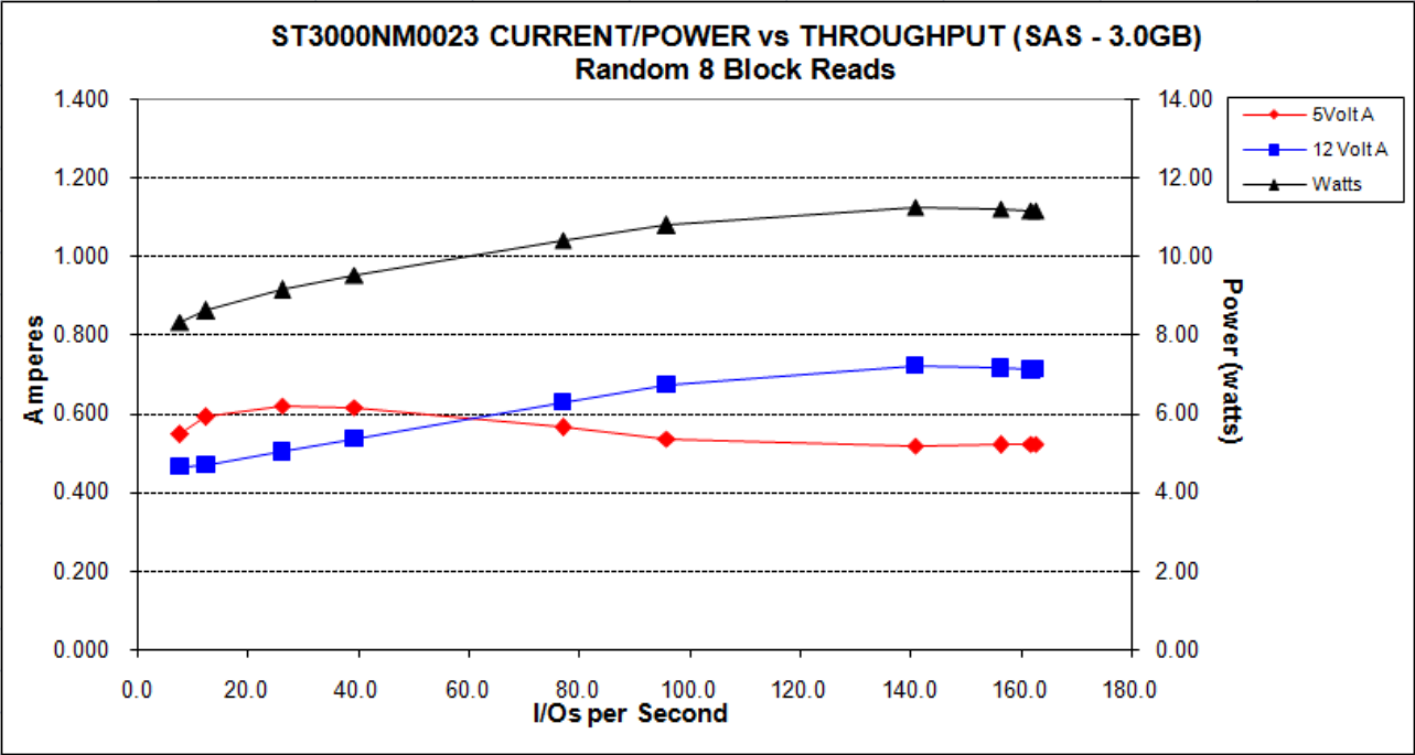
Figure 7. 3TB models (3Gb) DC current and power vs. input/output operations per second
