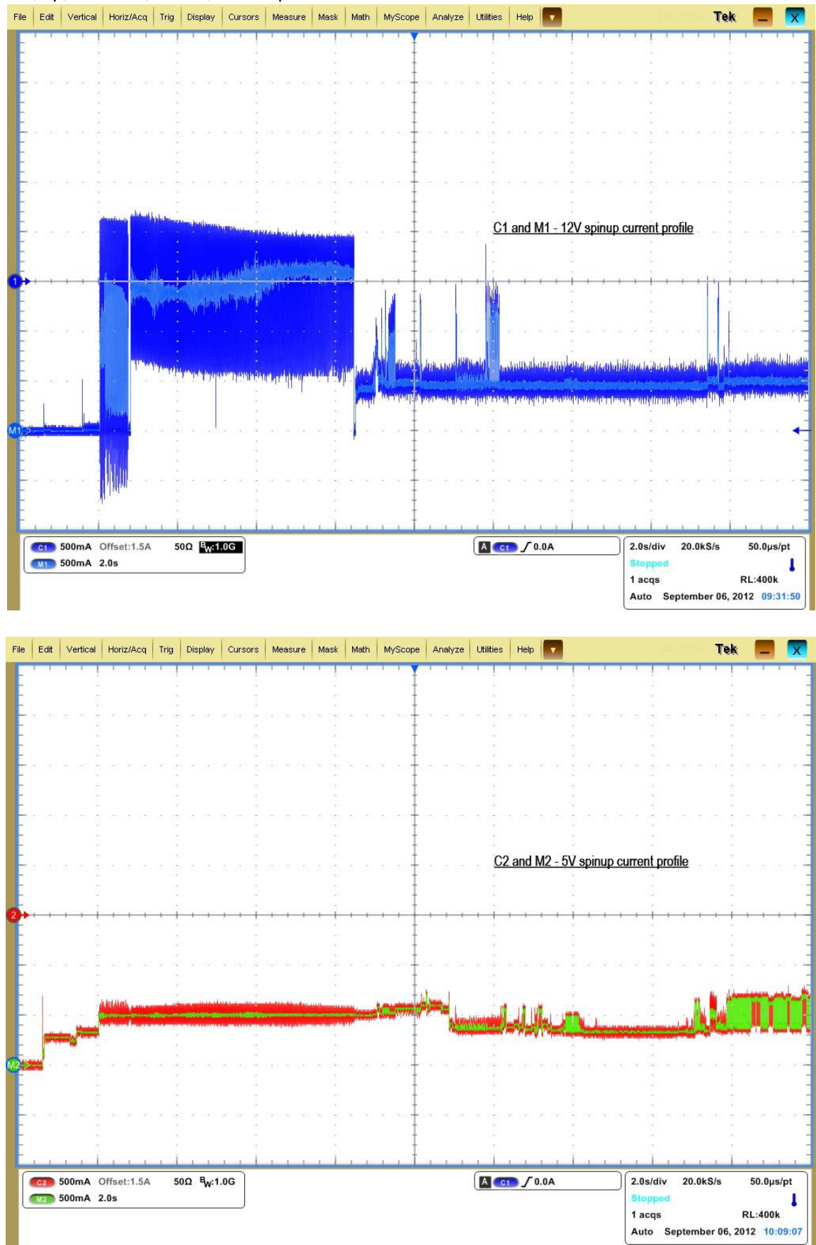
Figure 2. 3TB model current profiles
