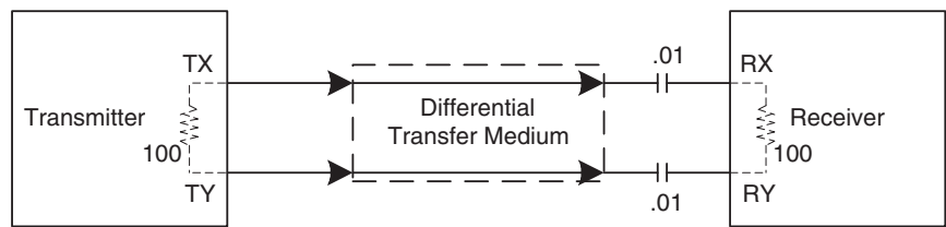
Figure 23. SAS transmitters and receivers
