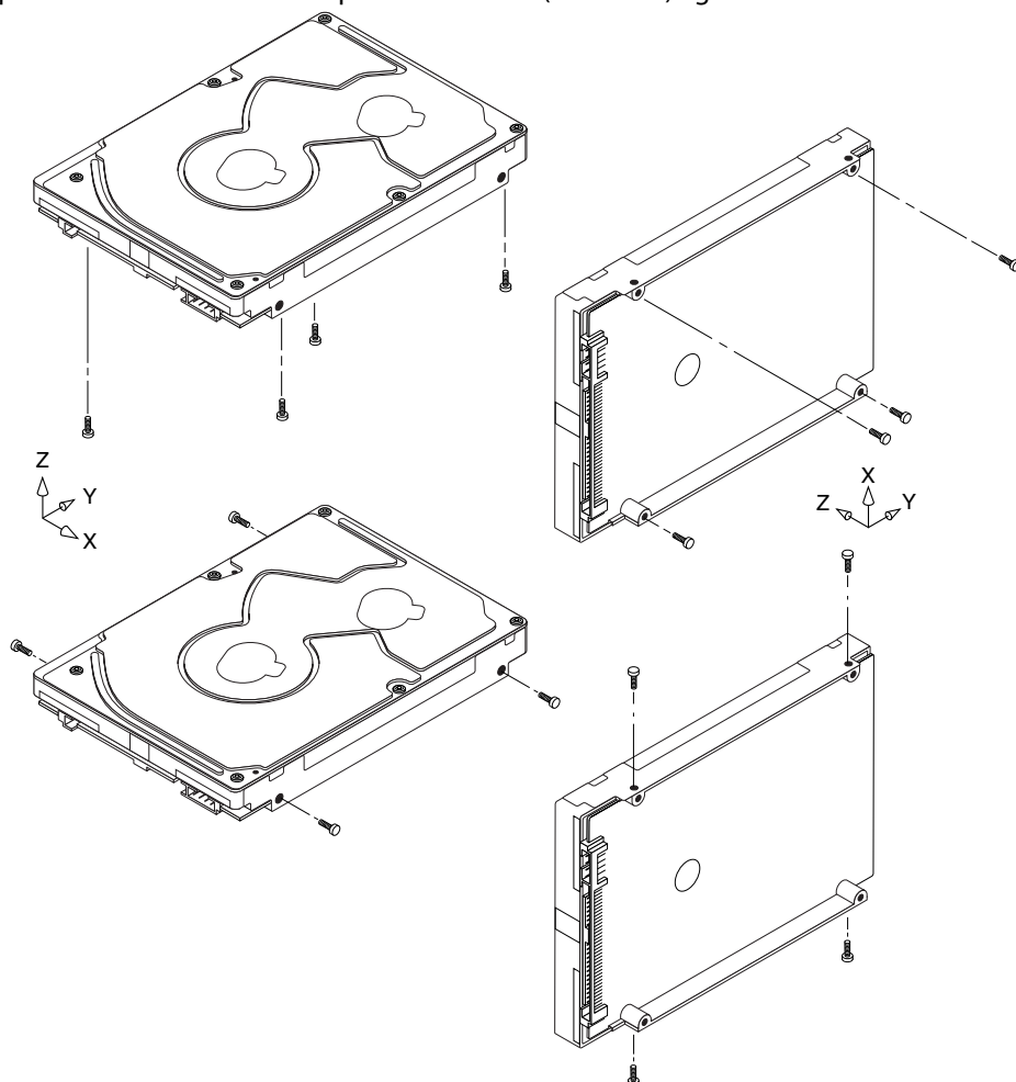
Figure 14. Recommended mounting
