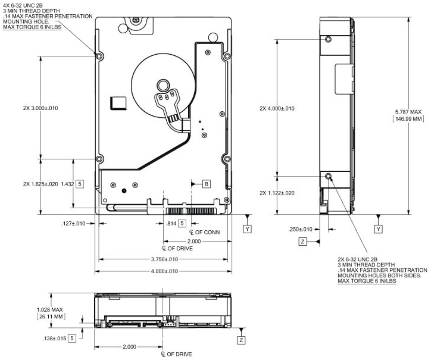
Figure 11. Mounting configuration dimensions (6TB models & ST5000NM0084)
