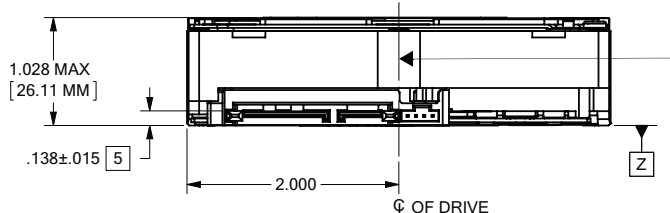
Figure 4. Mounting dimensions—top, side and end view (6TB)
