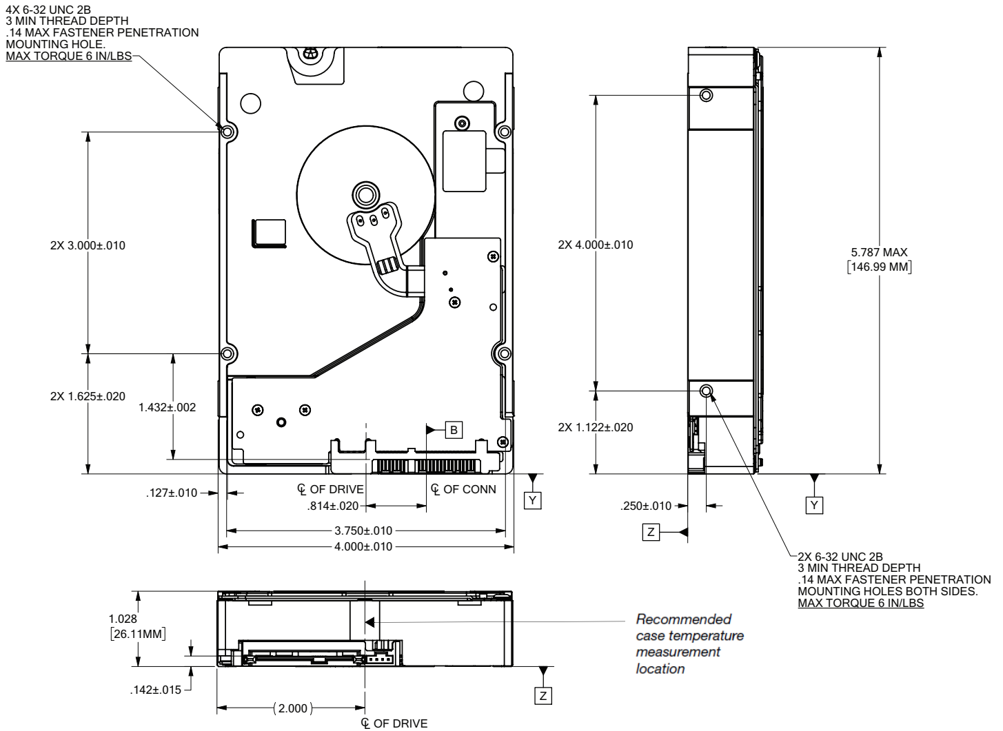
Figure 5. Mounting dimensions—top, side and end view (8TB)
