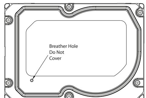
Figure 3. Breather hole location - top cover
