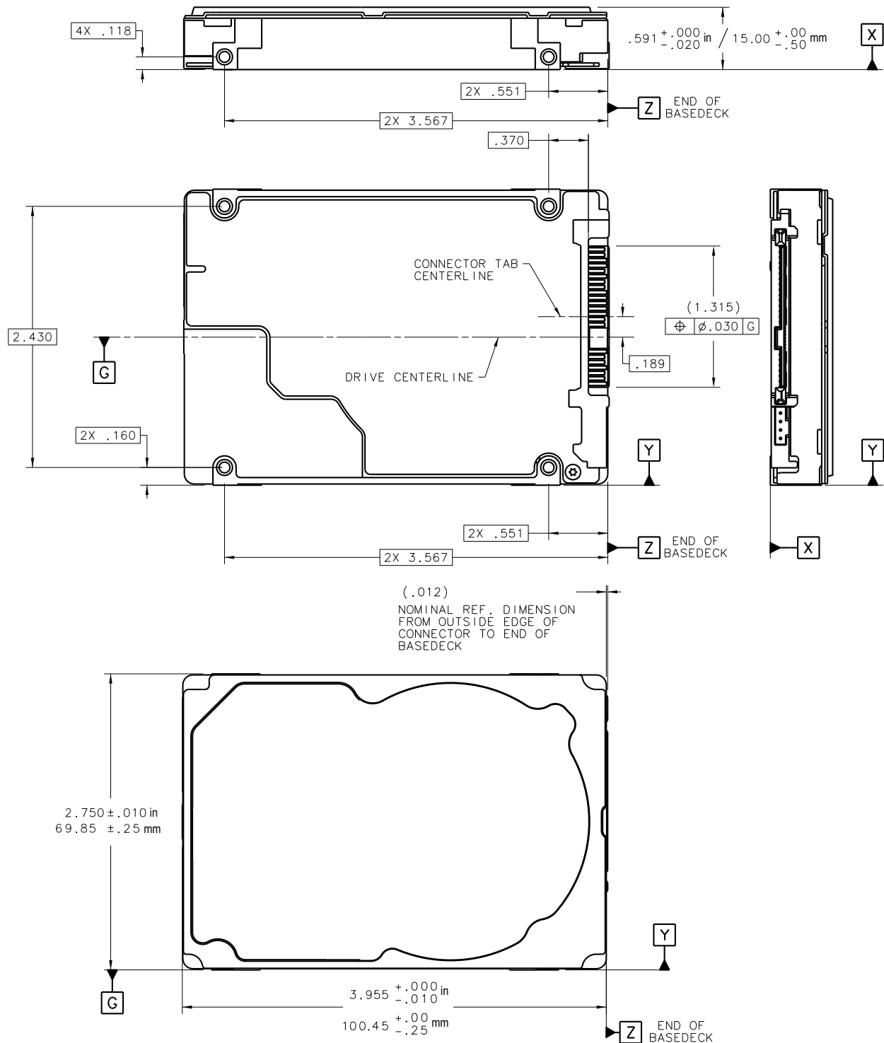
Figure 11. Dimensions
