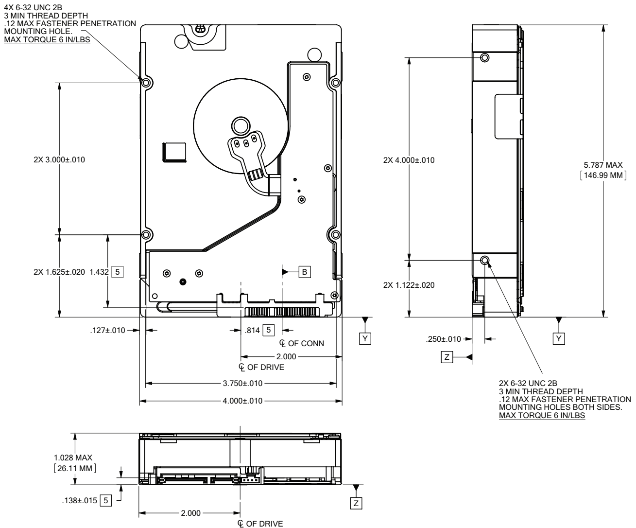
Figure 4. Mounting configuration dimensions (10TB & 8TB)
