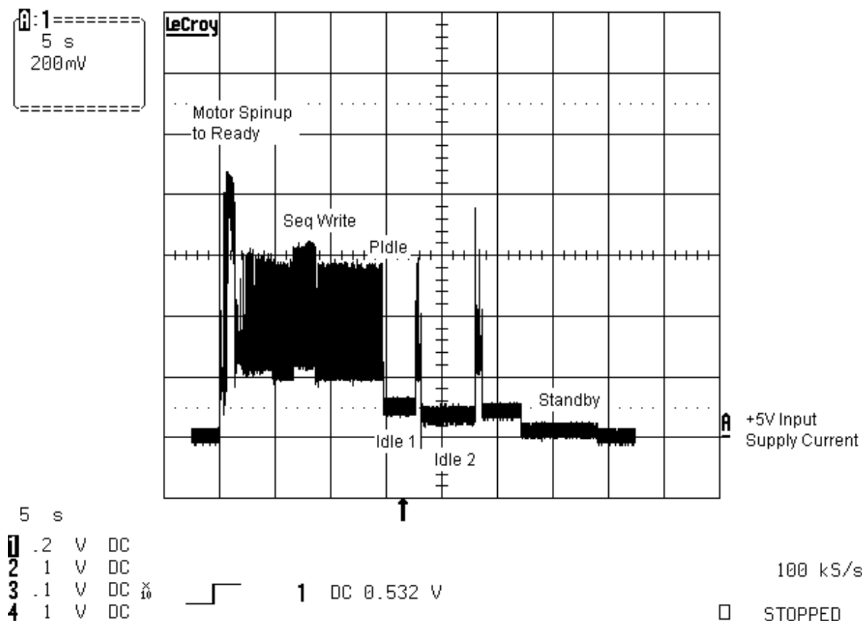
Figure 1 Typical 5V Startup and Operation Current Profile
