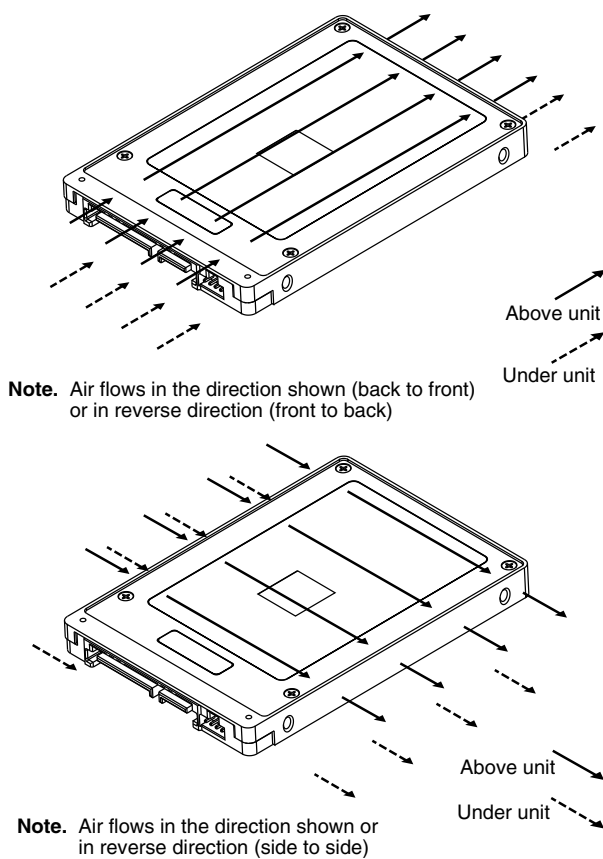
Figure 23. Air flow
