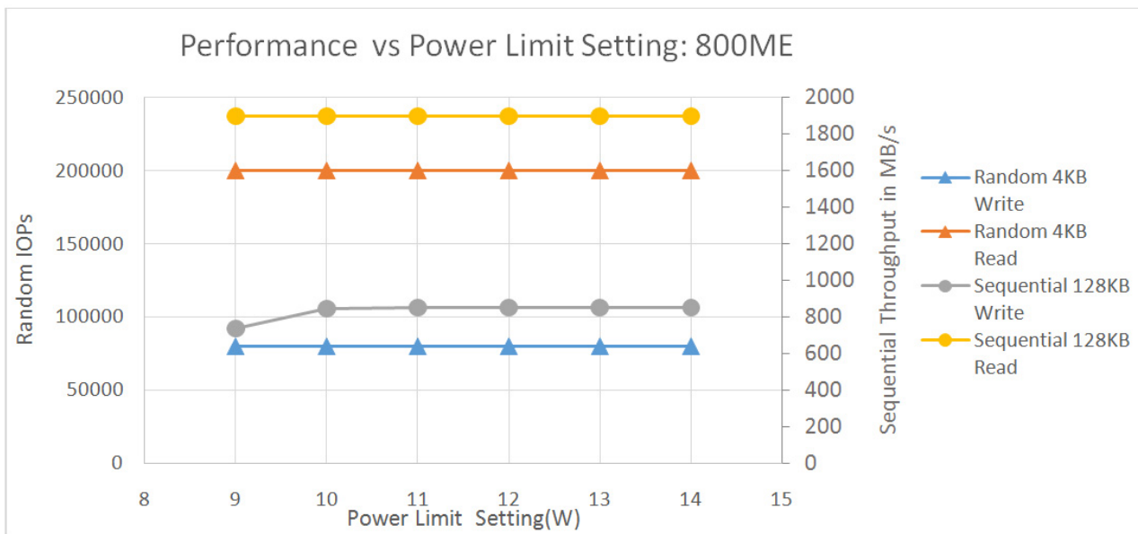
Figure 3. 800GB Mainstream Endurance: Performance vs Power Limit Settings IOPs chart
