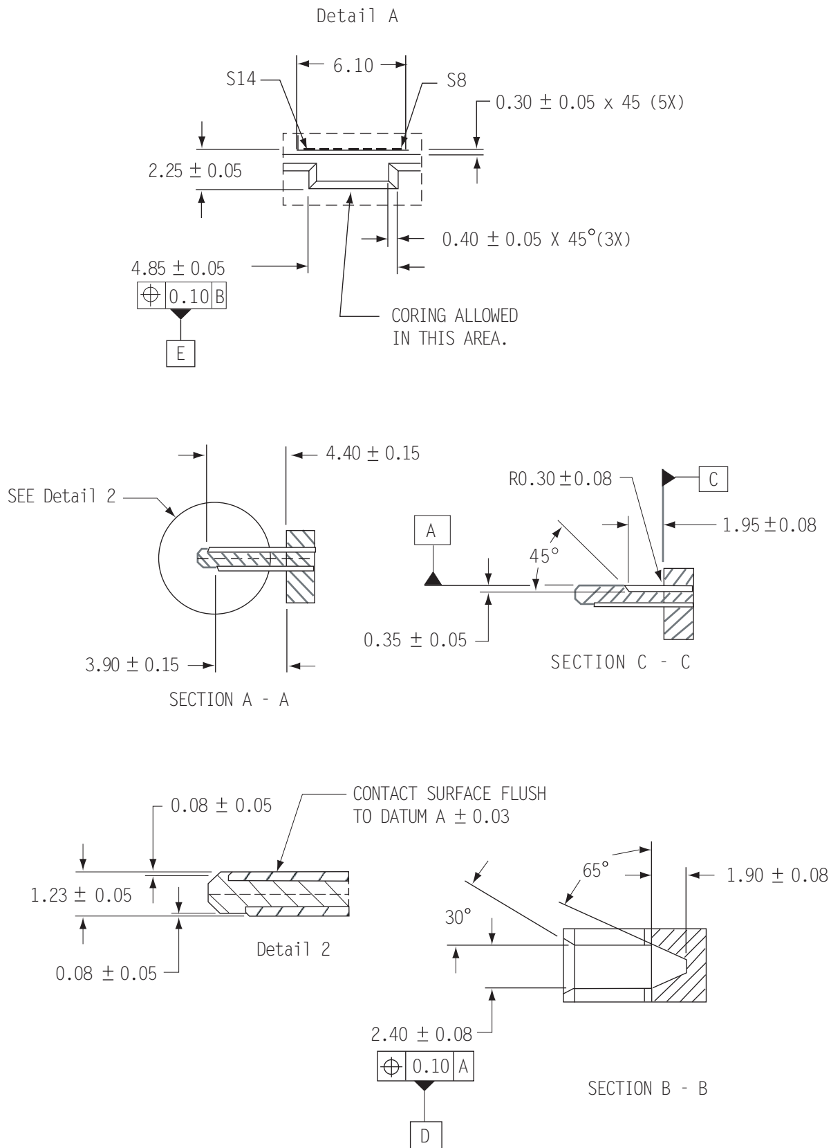
Figure 26. SAS device plug dimensions (detail)
