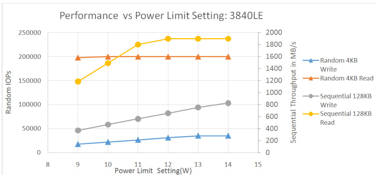
Figure 9. 3840GB Light Endurance: Performance vs Power Limit Settings IOPs chart
