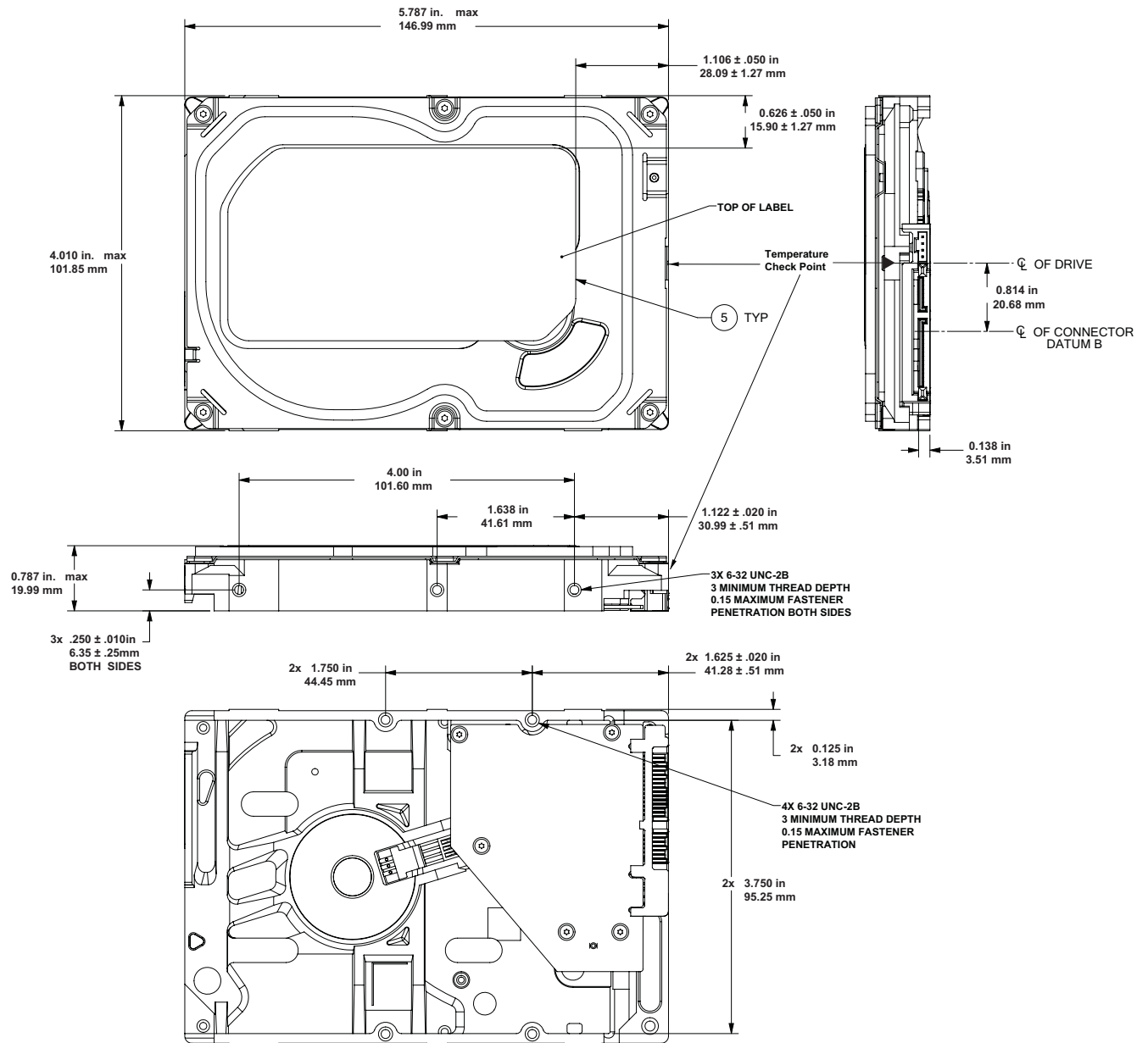
Figure 4 Mounting dimensions (1TB models)
