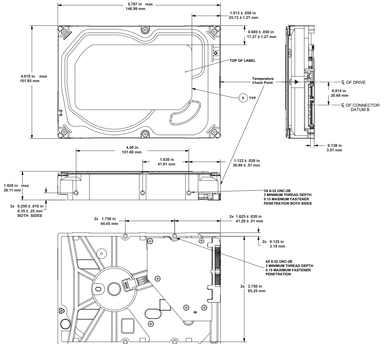
Figure 3 Mounting dimensions (4TB & 2TB models)
