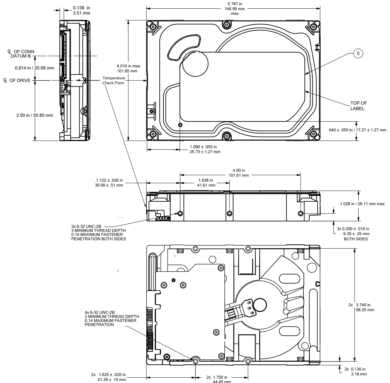
Figure 3 Mounting dimensions (4TB model)
