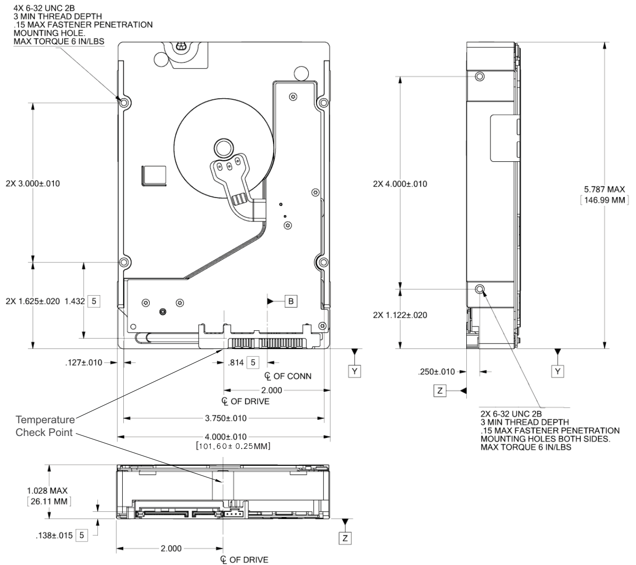
Figure 3 Mounting dimensions (6TB model)
