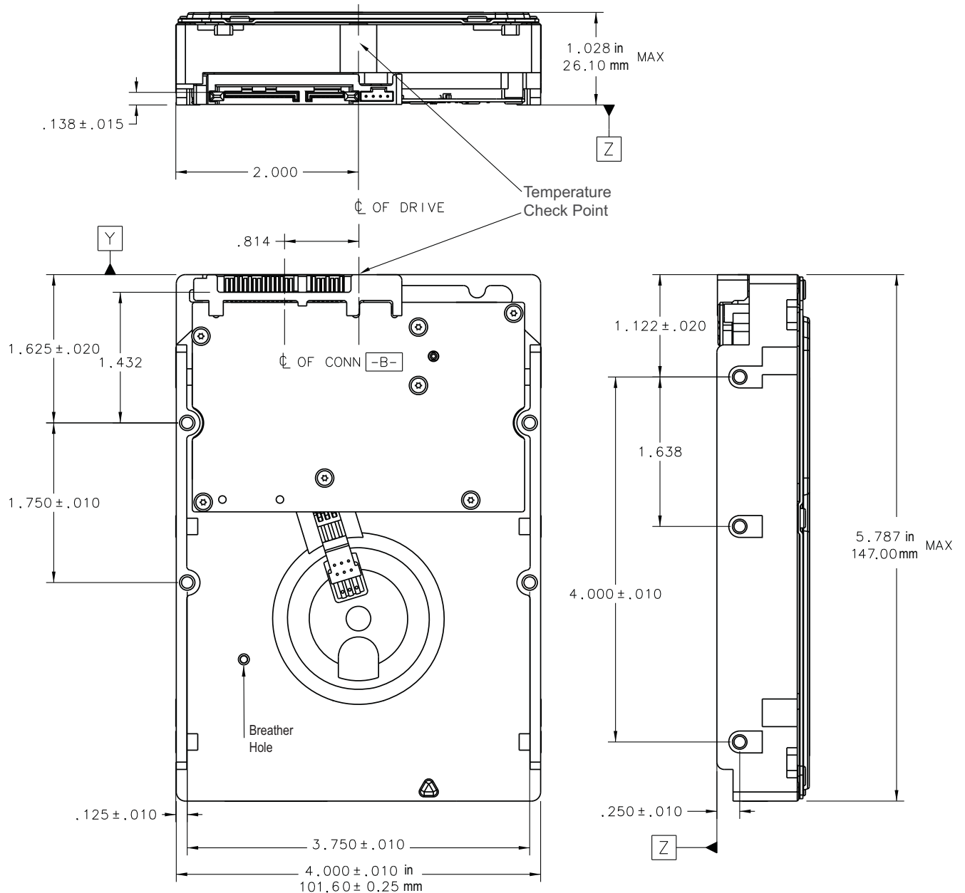
Figure 2 Mounting dimensions (5TB model)
