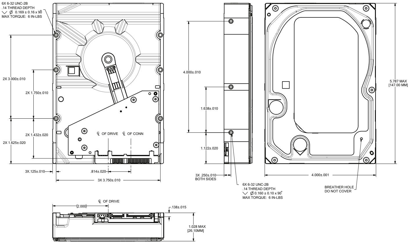
Figure 5. Mounting configuration dimensions 5-disk models
