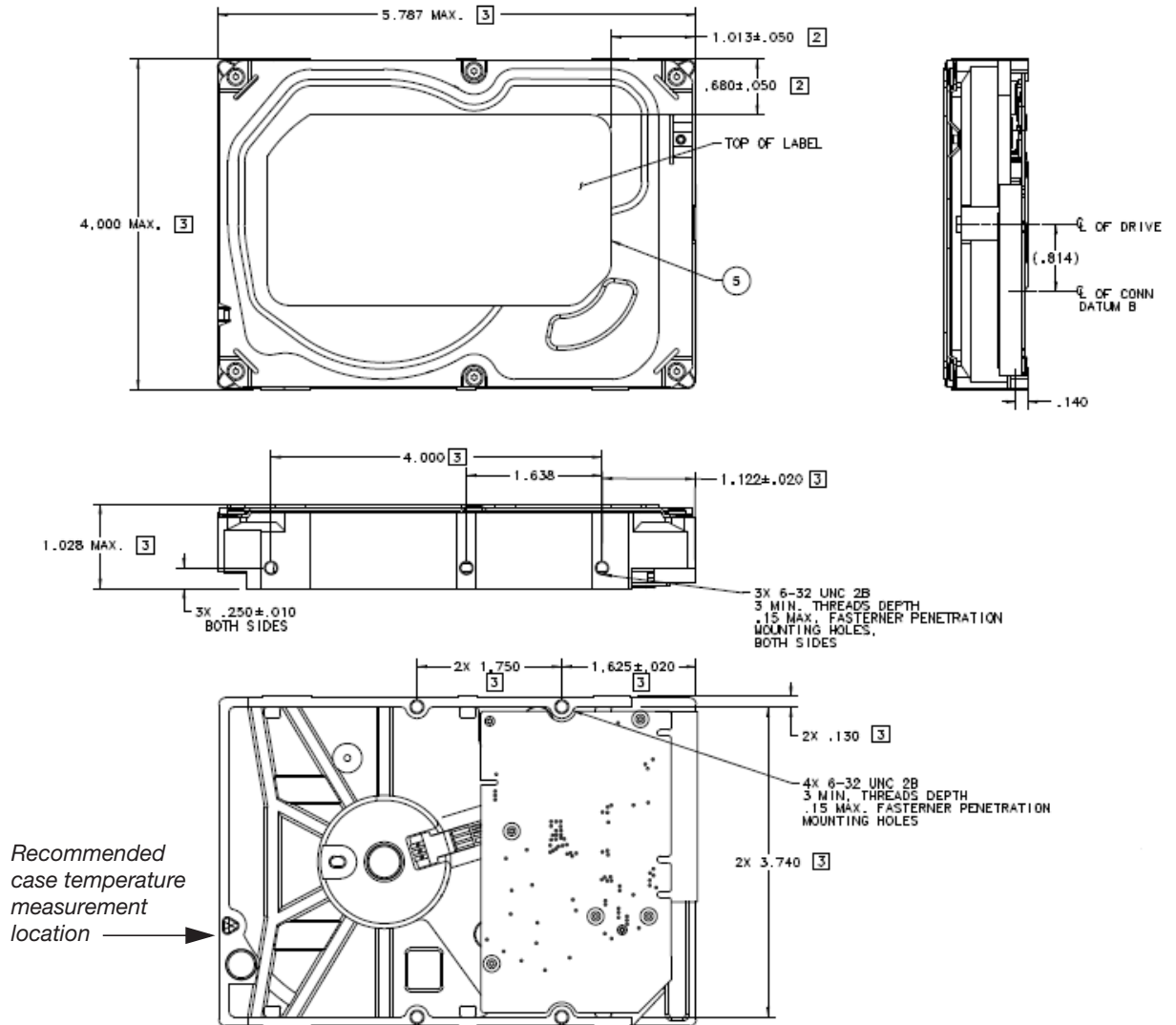
Figure 4 Mounting dimensions (2TB and 1.5TB models)
