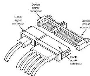
Figure 1 Attaching SATA cabling
