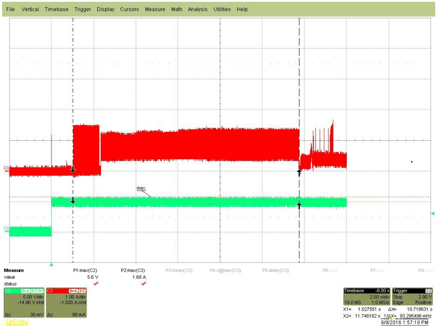
Figure 1. Typical 5V and 12V startup and operation current profiles (10TB & 8TB)
