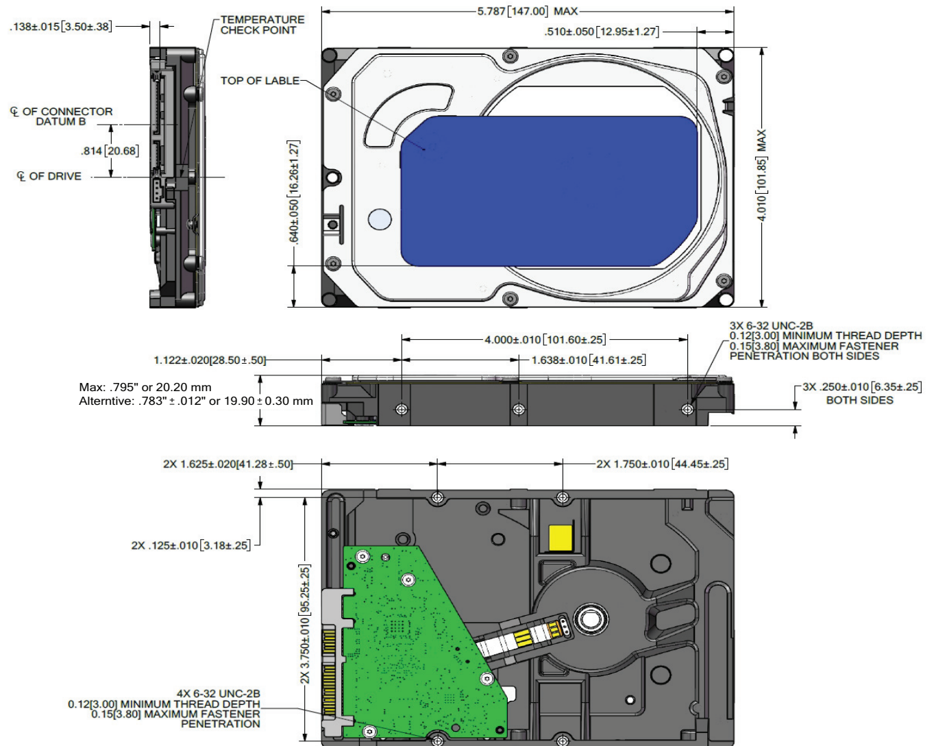
Figure 2 Mounting dimensions (1 and 2-disk models)
