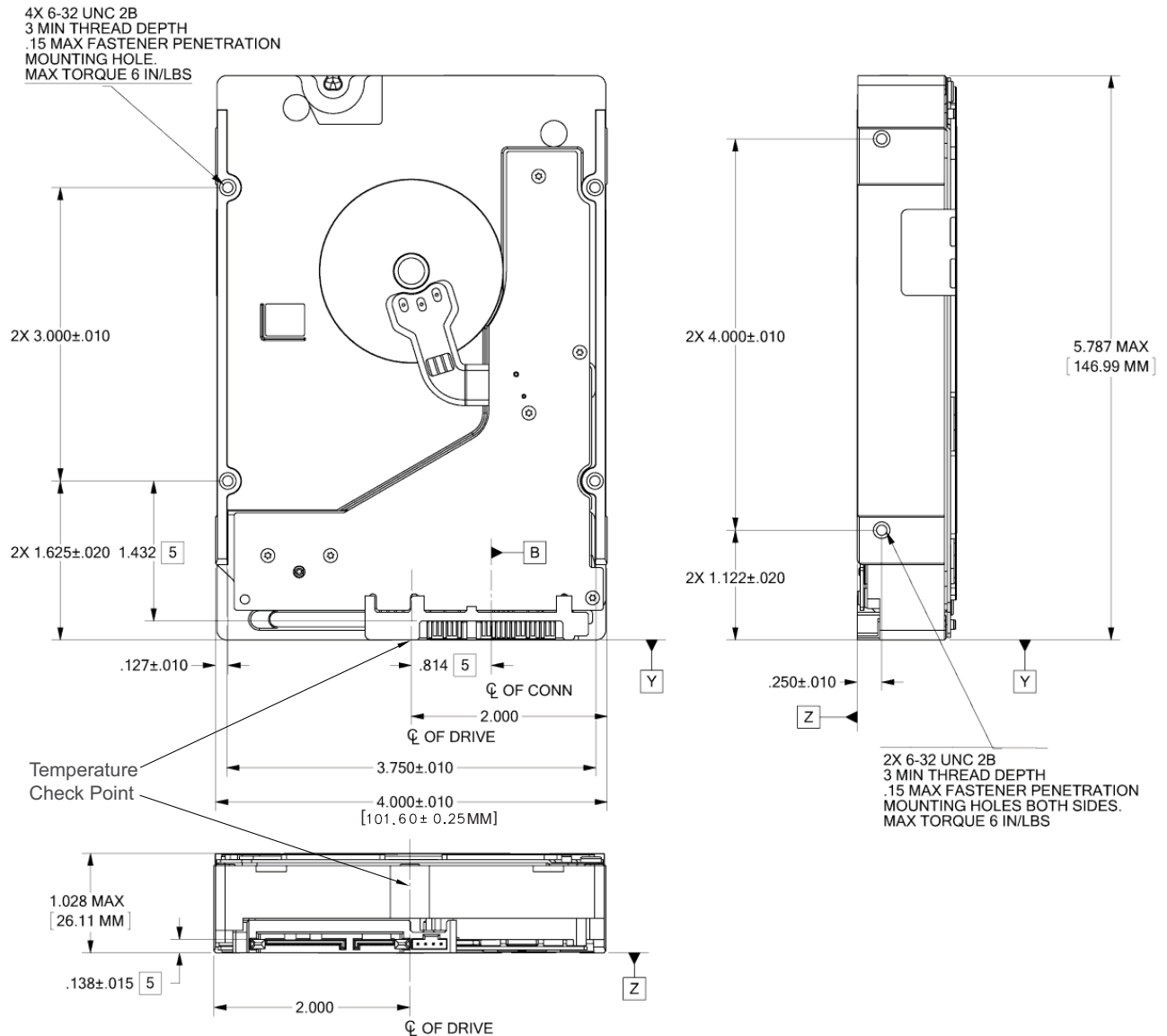
Figure 2 Mounting dimensions (5-6TB model)
