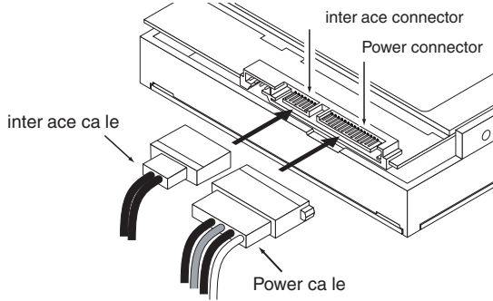
Figure 4. Attaching SATA cabling
