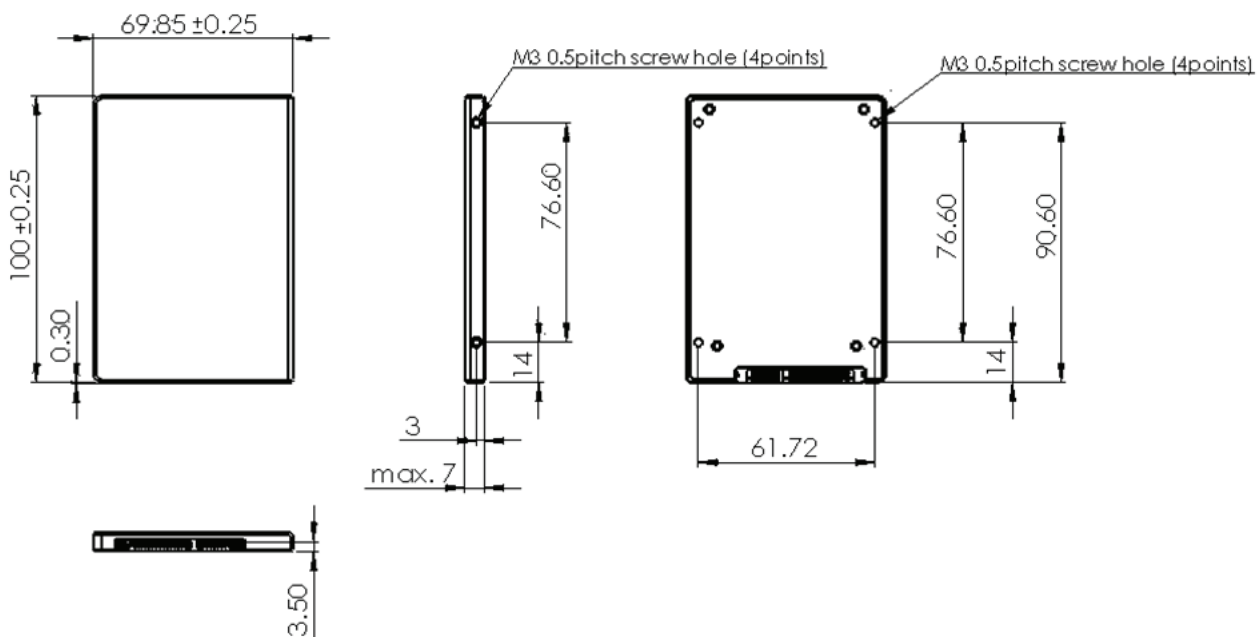
Figure 1 Dimensions
