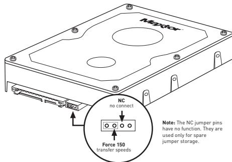
FIGURE 6B HARD DRIVE JUMPER PINS
