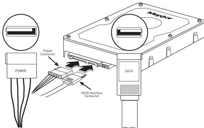
FIGURE 6A ATTACHING THE CABLES TO THE HARD DRIVE
