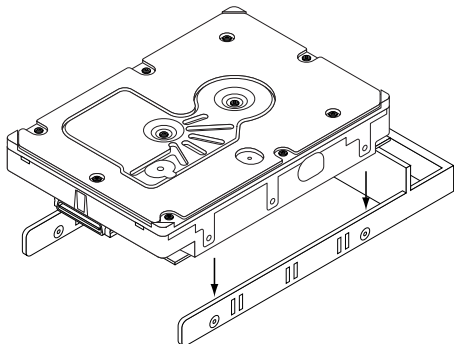
Figure 1. Sample drive carrier
