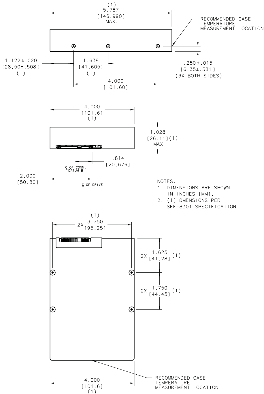
Figure 5. Mounting dimensions—top, side and end view
