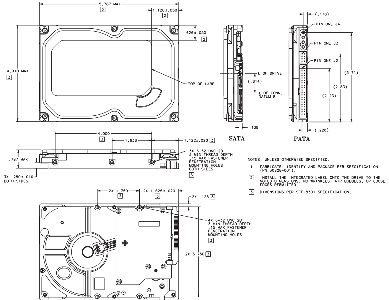
Figure 5. Mounting dimensions
