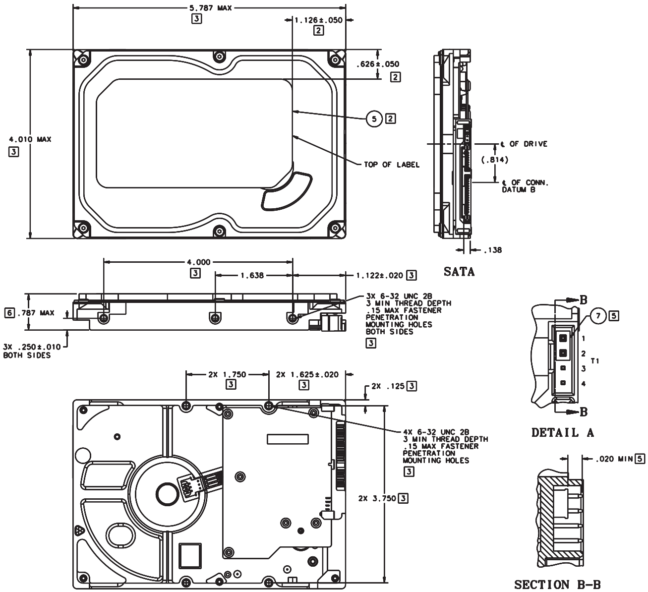
Figure 4. Mounting dimensions (320 and 160 GB models)
