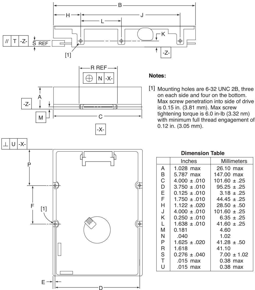
Figure 4. Mounting configuration dimensions
