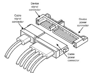
Figure 1 Attaching SATA cabling
