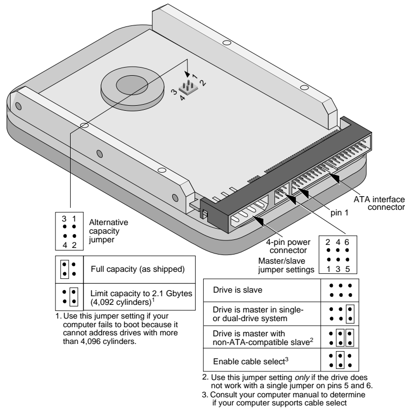
Figure 2. Master/slave jumpers and alternate capacity jumper for the ST33240A and ST32531A
