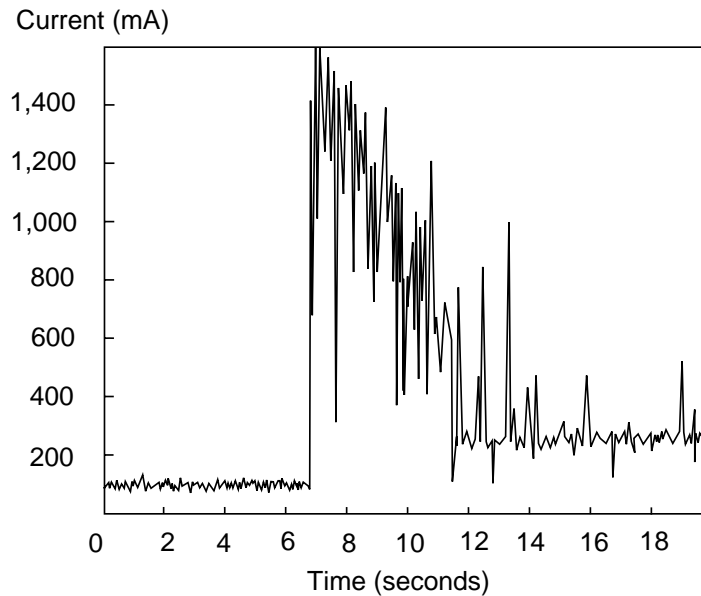
Figure 1. Typical startup and operation current profile
