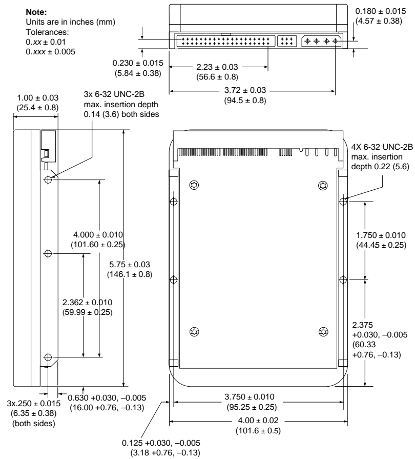
Figure 3. Mounting dimensions for the ST33240A and ST32531A—top, side and end view
