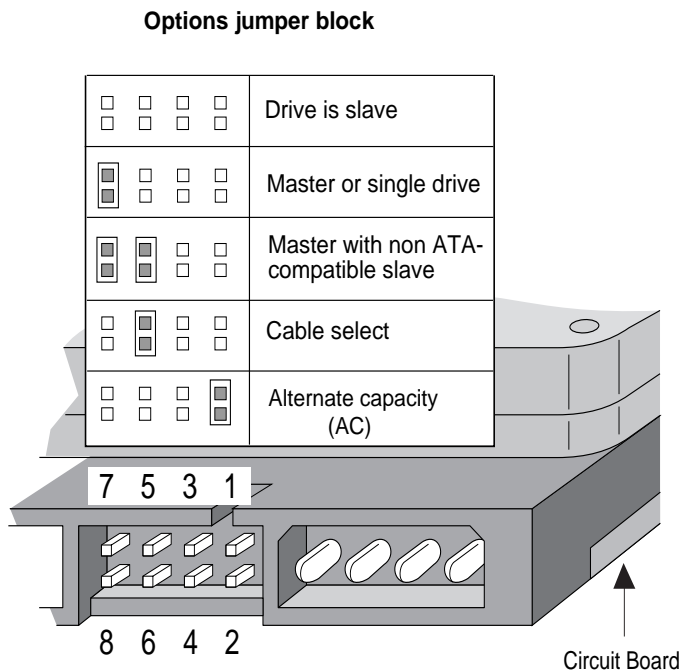
Figure 2. Master/slave jumper settings
