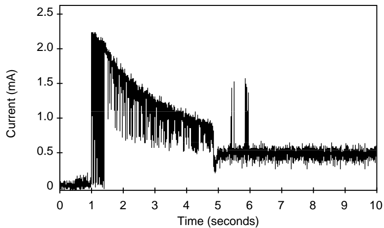
Figure 1. Typical startup and operation current profile
