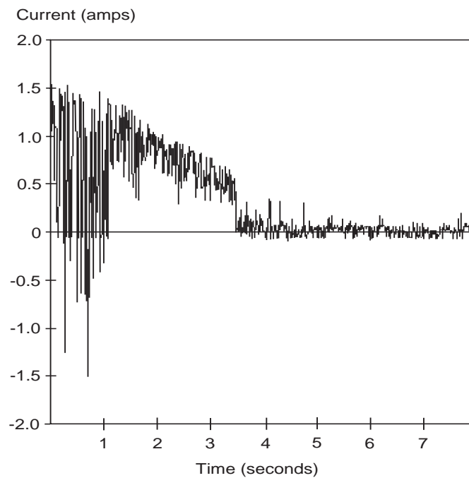
Figure 1. Typical startup and operation current profile
