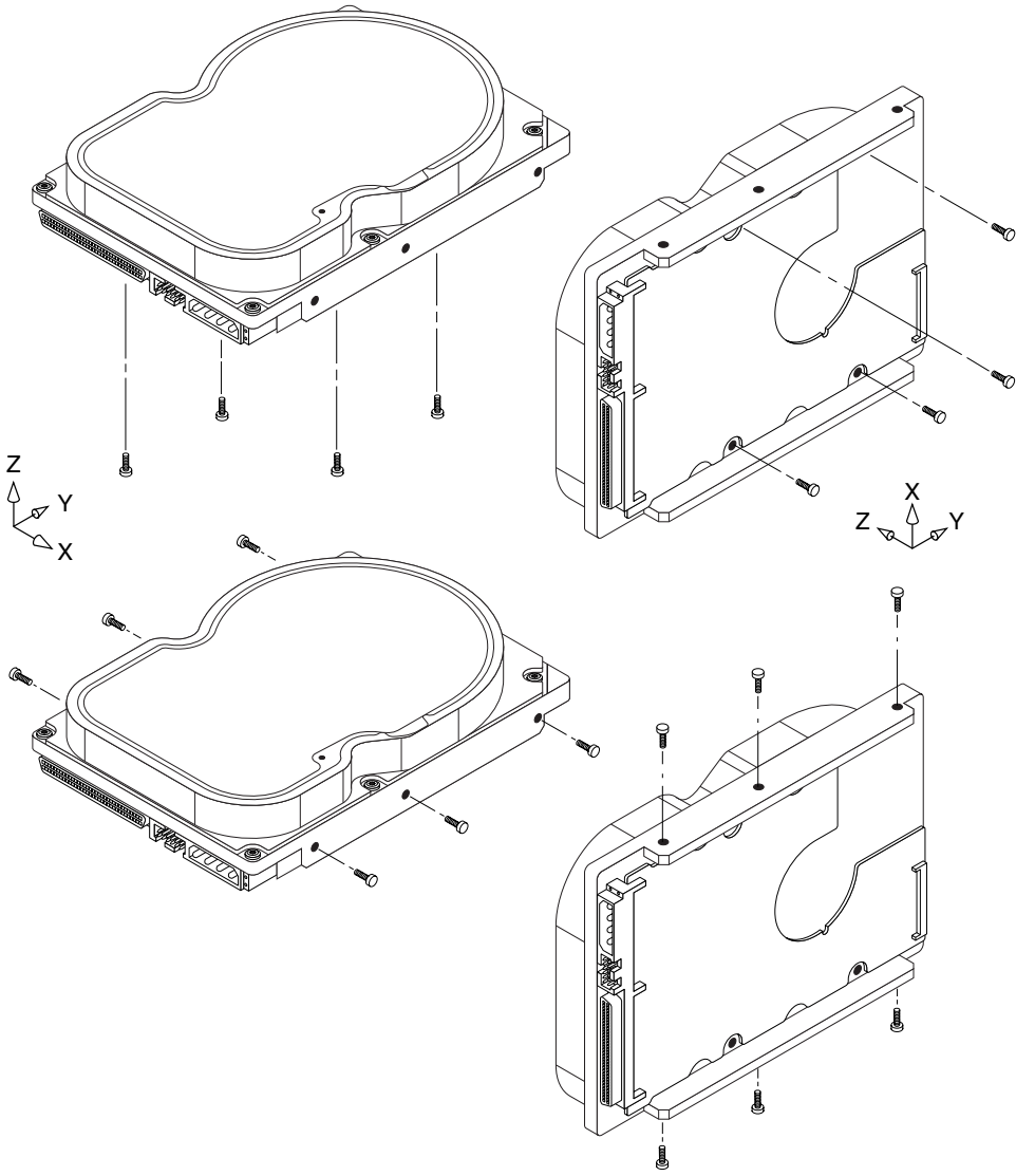
Figure 11. Recommended mounting
