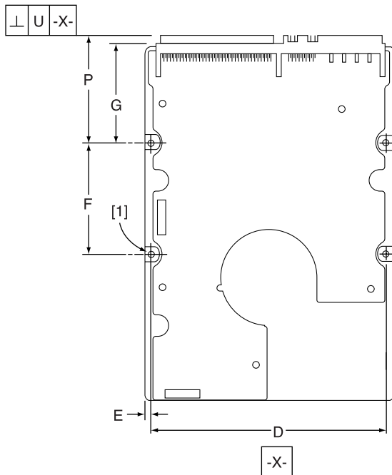
Figure 12. LW and W mounting configuration dimensions
