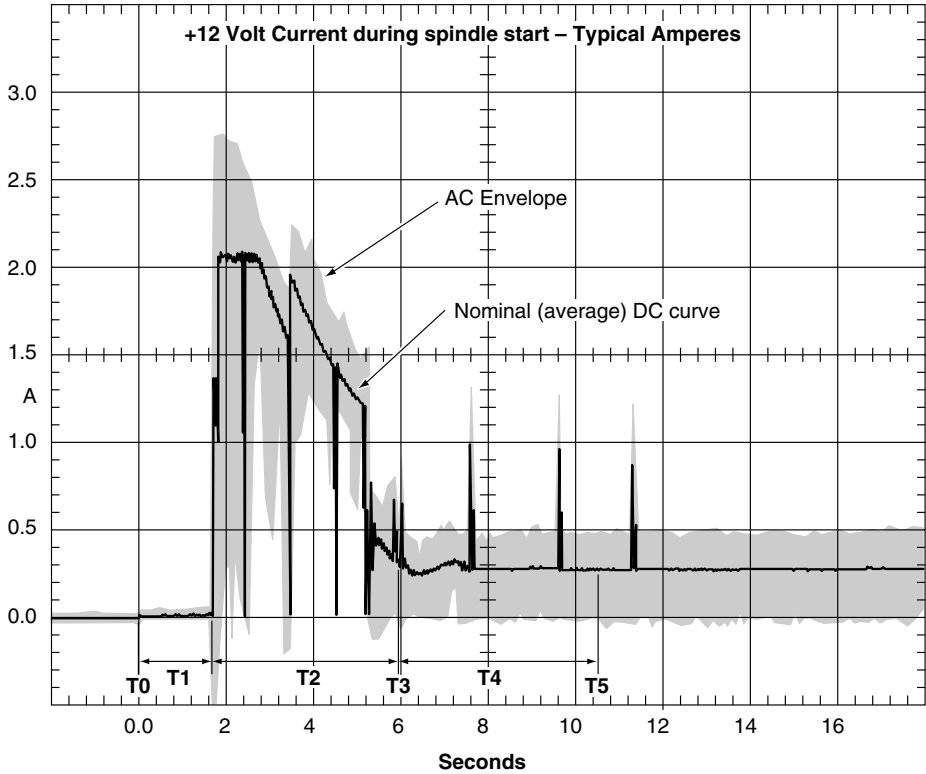
Figure 3. Typical ST336737 drive +12 V current profile
